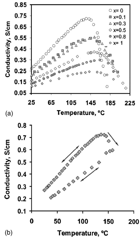
FIG. 2. (a) Conductivity vs temperature of \text{Ca}_{12-x}\text{Mg}_x\text{Al}_{14}\text{O}_{33} ( x=0, 0.1, 0.3, 0.5, 0.8, 1 ) and (b) conductivity vs temperature of pure mayenite ( \text{Ca}_{12}\text{Al}_{14}\text{O}_{33} ) showing irreversible loss of conductivity above the decomposition temperature (135 °C).
