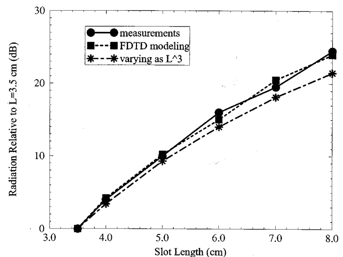
Fig. 12. The relation of EMI to slot length for a single slot.
