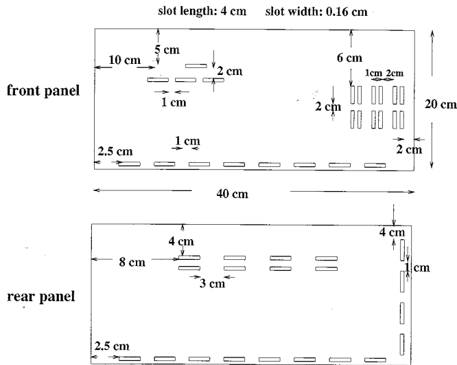
Fig. 3. The panels used in the S-1000E test enclosure with 4-cm slots as radiators.
