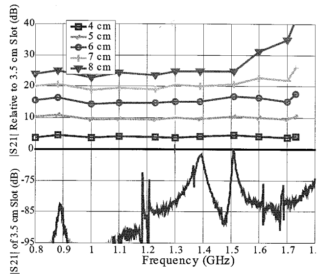
Fig. 11. The radiation from a single slot with varying slot length.
