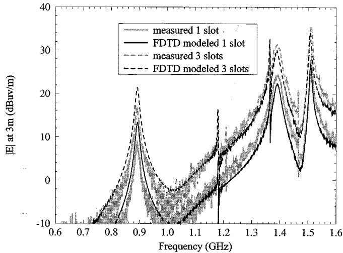
Fig. 13. The EMI from side-by-side multiple slots.
