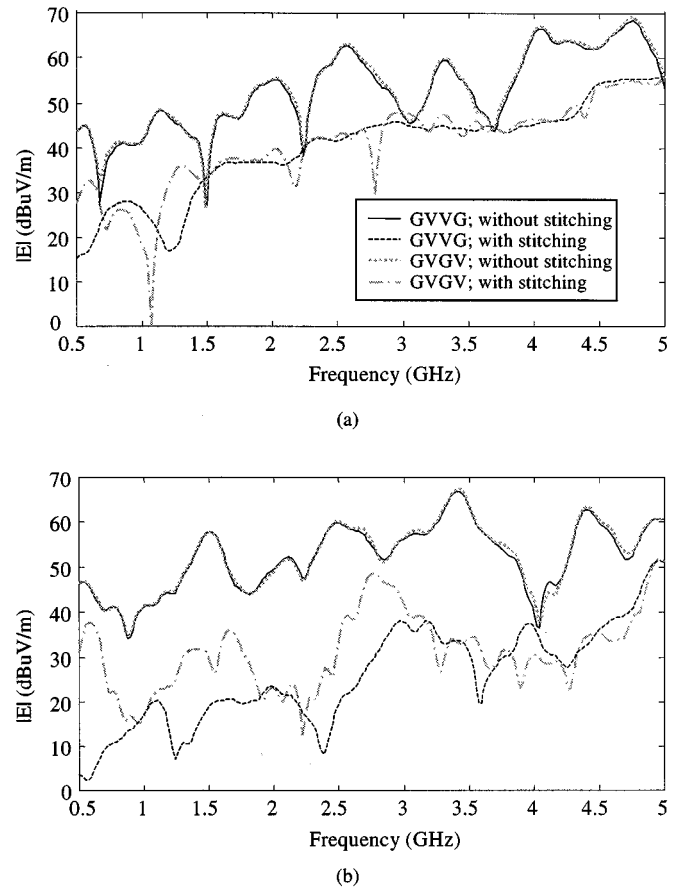
Fig. 13. Modeled EMI at 3 m for the cases with and without stitching for the GVVG and GVGv configurations with the source on top of all planes. (a) E_x polarization. (b) E_y polarization.
