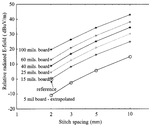
Fig. 18. The EMI at 3 m as a function of stitch spacing for different layer thicknesses.
