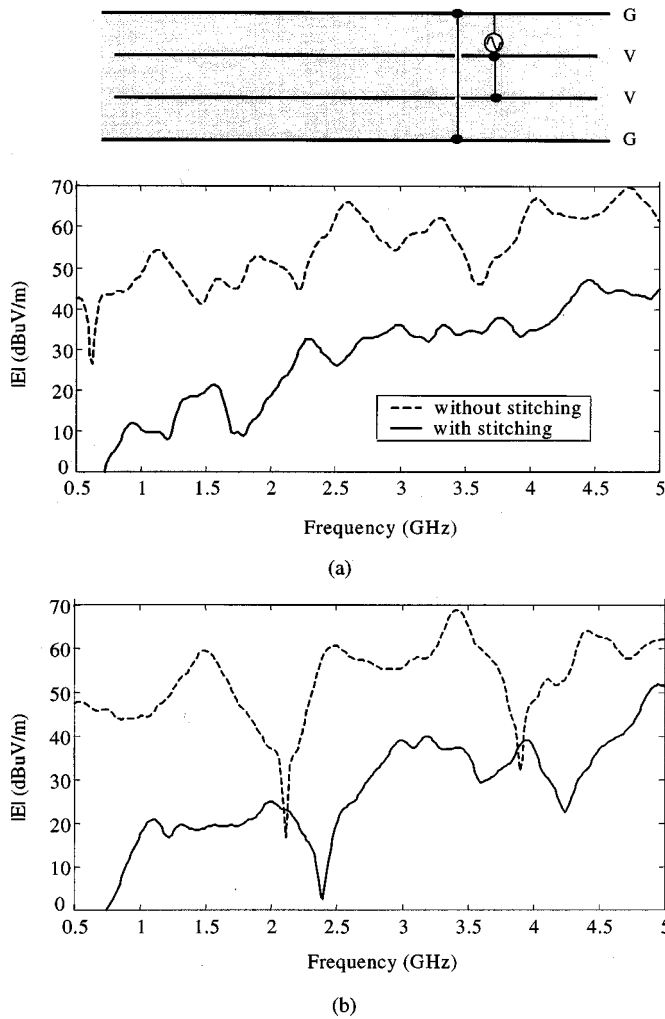
Fig. 14. Modeled EMI at 3 m for the cases with and without stitching for the GVVG configuration with a source placed in between planes. (a) E_x polarization. (b) E_y polarization.
