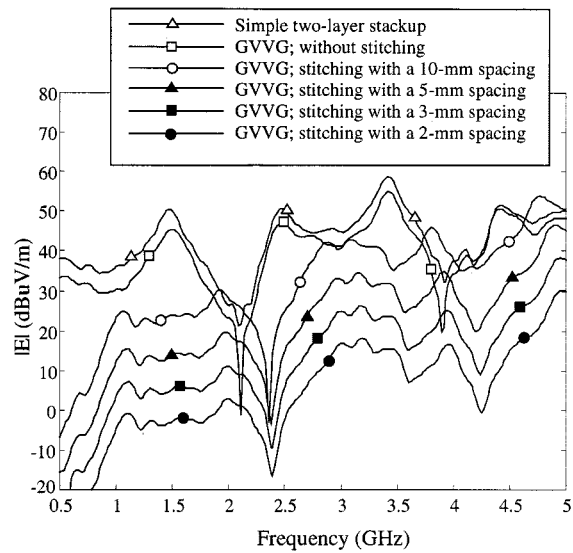
Fig. 16. The modeled EMI at 3 m for different stitching cases, together with the case without stitching and a two-layer stack-up. The layer thickness was 25 mil for all cases.
