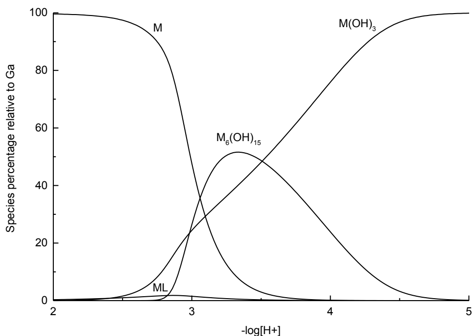
Figure 3: Simulated distribution of the Ga(III) into its free, complexed and hydroxides species as a function of pH, with Ga(III) = 2 \text{ mmol.dm}^{-3} and ACT = 2 \text{ mmol.dm}^{-3} .
