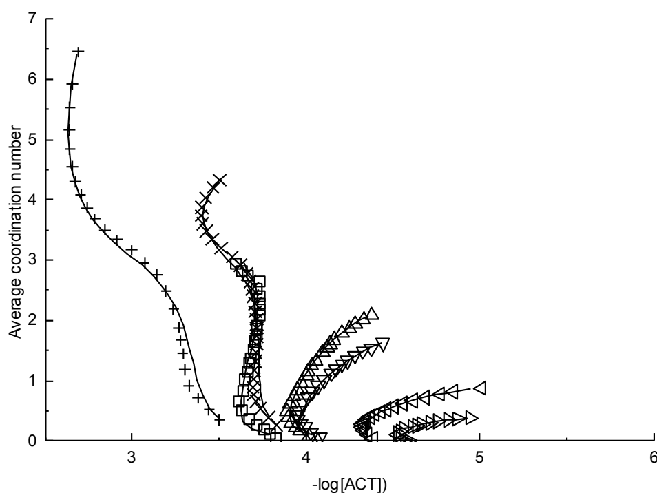
Figure 2: Formation curves relative to Ga(III) –ACT mixture. Symbols as in Table I. Solid lines represent the corresponding simulated protonation curves as obtained by means of SIMDIS using data in Table II.
