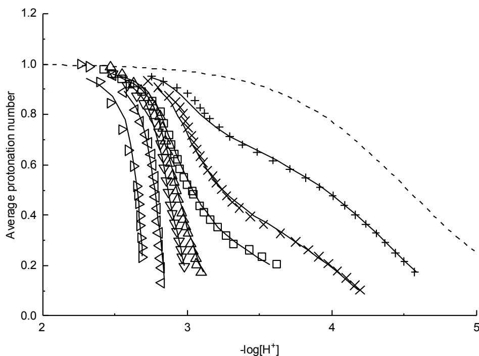
Figure 1: Protonation curves relative to Ga(III) -ACT mixture. Symbols as in Table I. Dashed line represents the calculated protonation curve of ACT in the absence of Ga(III). Solid lines are theoretical curves calculated with the help of SIMDIS program using results of Table II.
