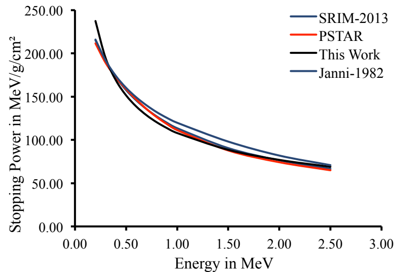
Figure 4: A graph of Stopping Power of protons versus energy in Germanium for Janni-1982, SRIM-2013, PSTAR codes and New Empirical relation.
