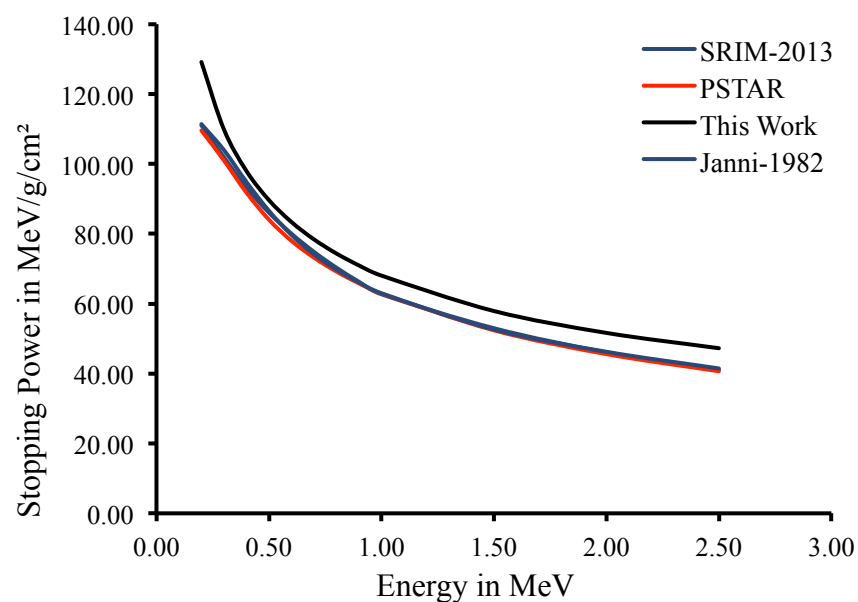
Figure 2: A graph of Stopping Power of protons versus energy in Copper for Janni-1982, SRIM-2013, PSTAR codes and Modified Empirical relation.
