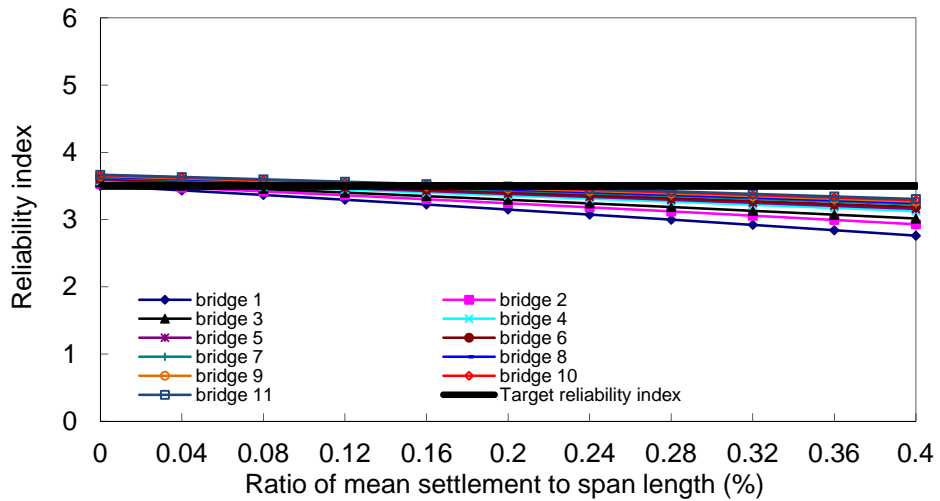
(c) Reliability indices for shear
