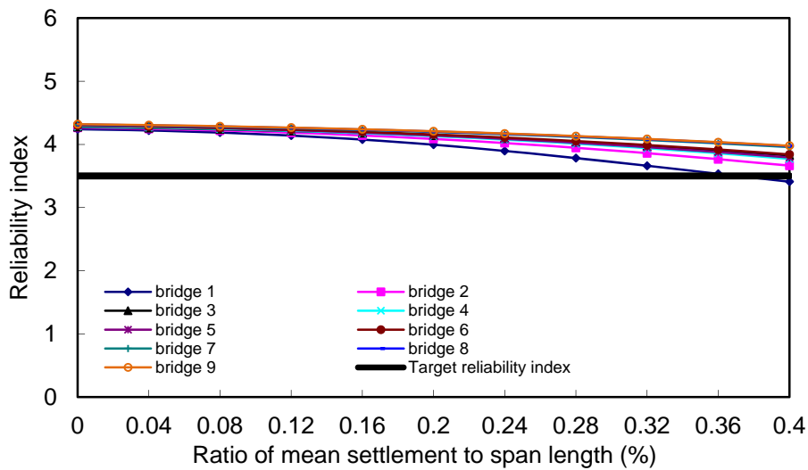
Figure 5.11 Reliability indices of 4-span bridges (No.23 to No.31 in Table 2.3): Case 3
