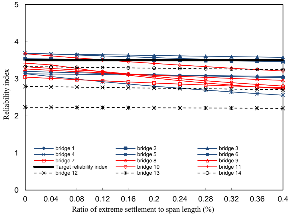
(c) Reliability indices for shear
