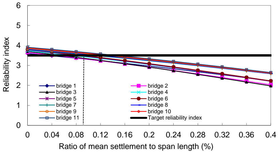
(b) Reliability indices for positive moment
