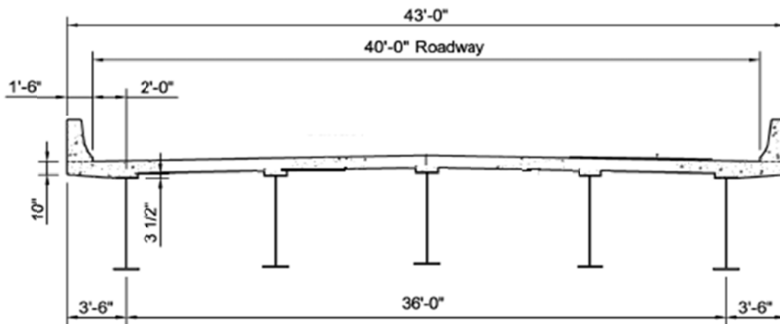
Figure 2.18 Cross section of new girder bridges
