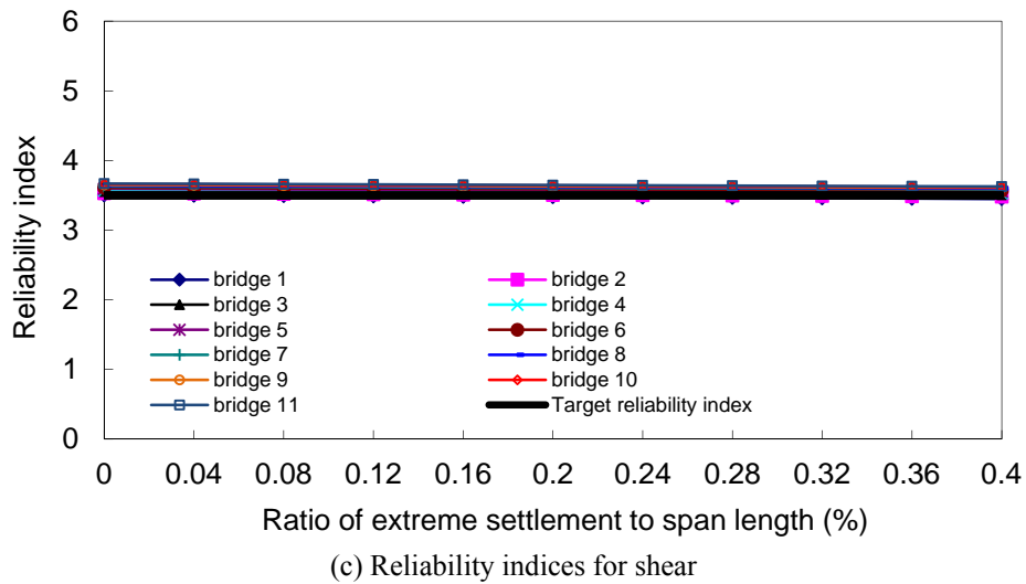
Figure 5.24 Reliability indices of 2-span bridges (No.1 to No.11 in Table 2.3): Case 8
