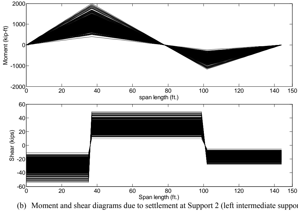
Figure 2.7 Bridge A4058 under a random support settlement: mean=1 in. and COV=0.25
