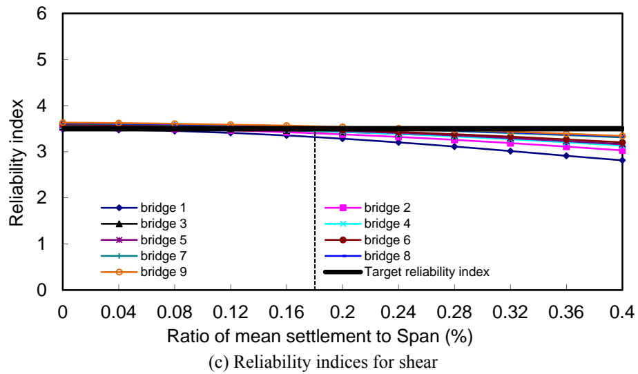
Figure 5.23 Reliability indices of 4-span bridges (No.23 to No.31 in Table 2.3): Case 7
