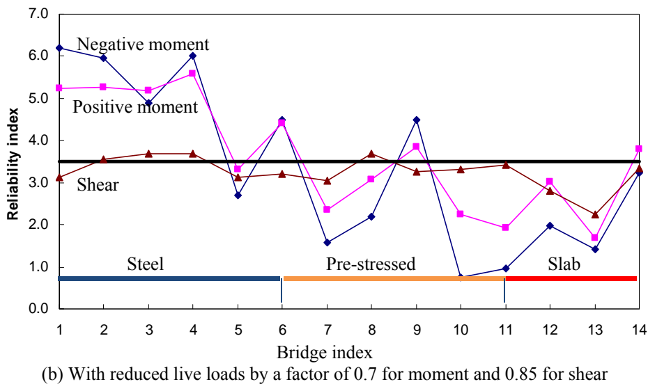
Figure 5.37 Reliability indices of 14 existing bridges without settlement effects
