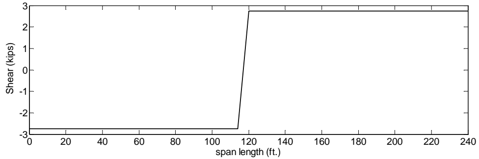
(b) Shear diagram
