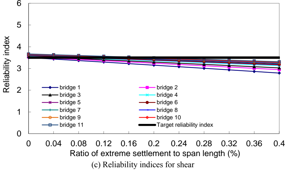
Figure 5.18 Reliability indices of 2-span bridges (No.1 to No.11 in Table 2.3): Case 6
