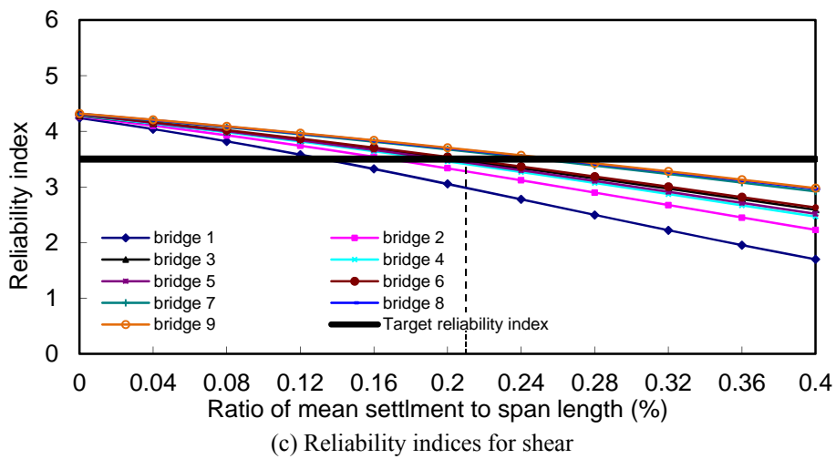
Figure 5.5 Reliability indices of 4-span bridges (No.23 to No.31 in Table 2.3): Case 1
