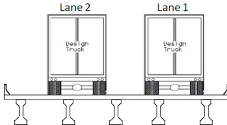
Figure 5.1 Multiple-lane load
