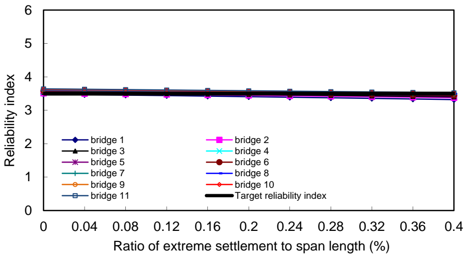
Figure 5.25 Reliability indices of 3-span bridges (No.12 to No.22 in Table 2.3): Case 8
