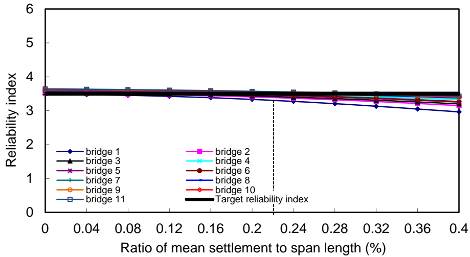
Figure 5.22 Reliability indices of 3-span bridges (No.12 to No.22 in Table 2.3): Case 7
