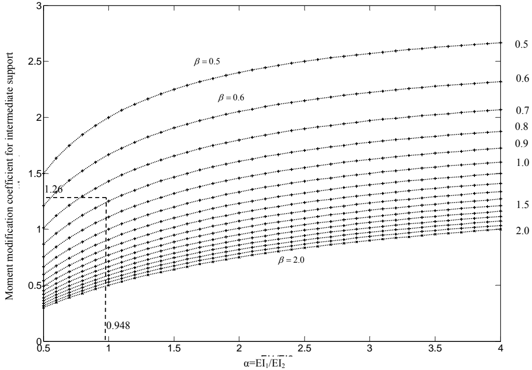
(b) Due to a unit settlement at the intermediate support Figure 2.14 f(\alpha, \beta) for 2-span continuous girders
