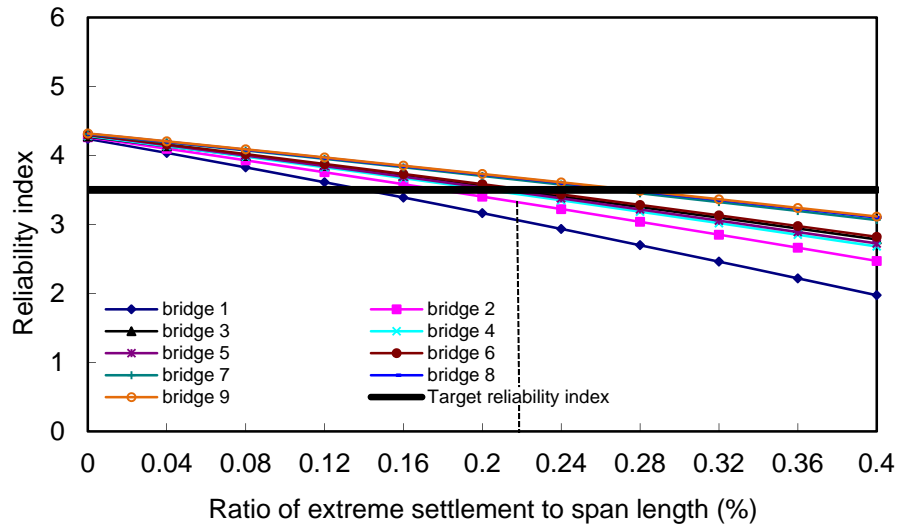
Figure 5.8 Reliability indices of 4-span bridges (No.23 to No.31 in Table 2.3): Case 2
