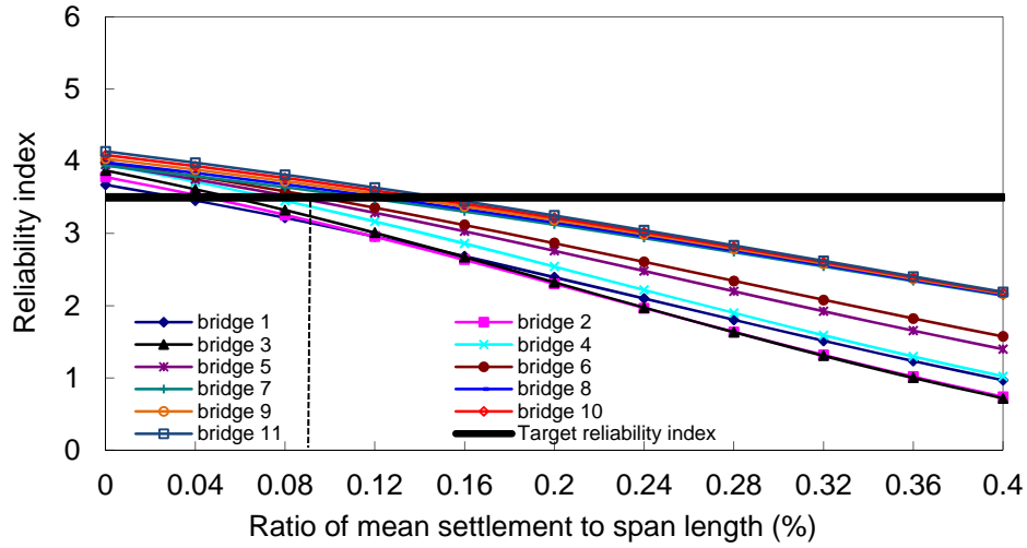
(a) Reliability indices for negative moment
