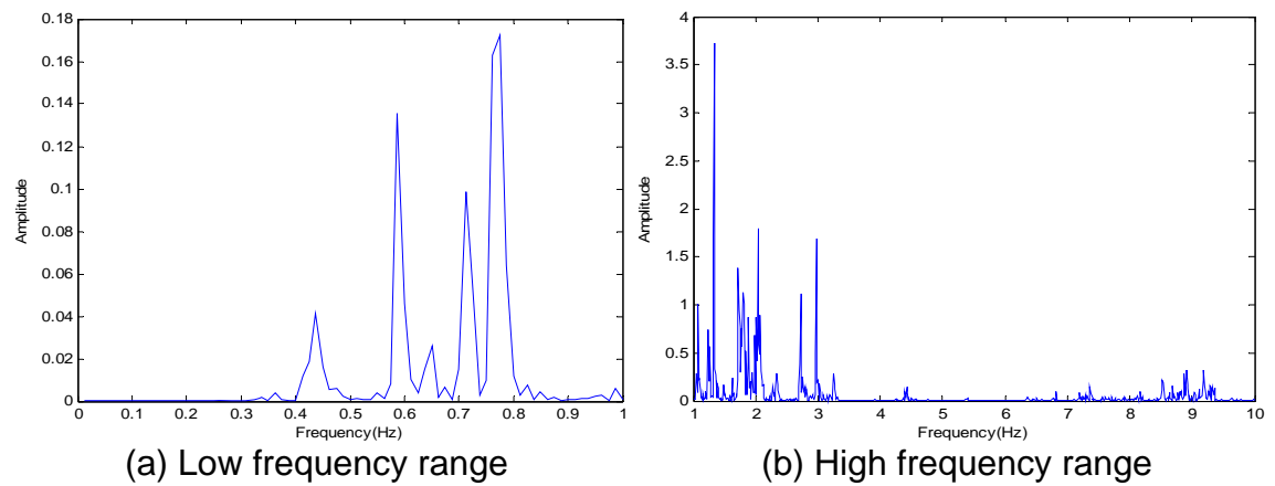
Figure 3.22 Fourier spectrum of acceleration at HNZ-L6
