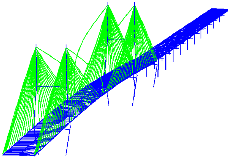
Figure 5.22 21 st mode shape (0.962Hz)
