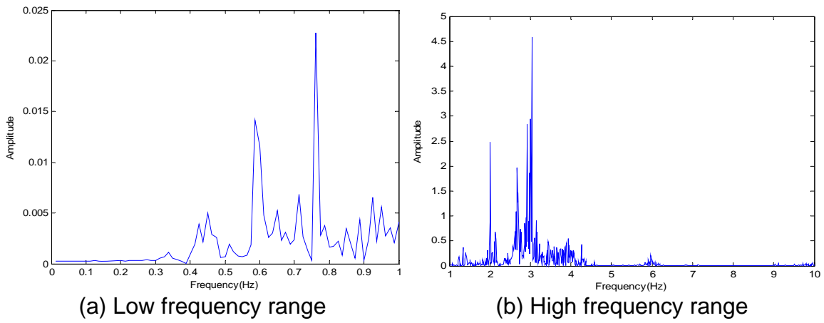
Figure 3.21 Fourier spectrum of acceleration at HN3-T3
