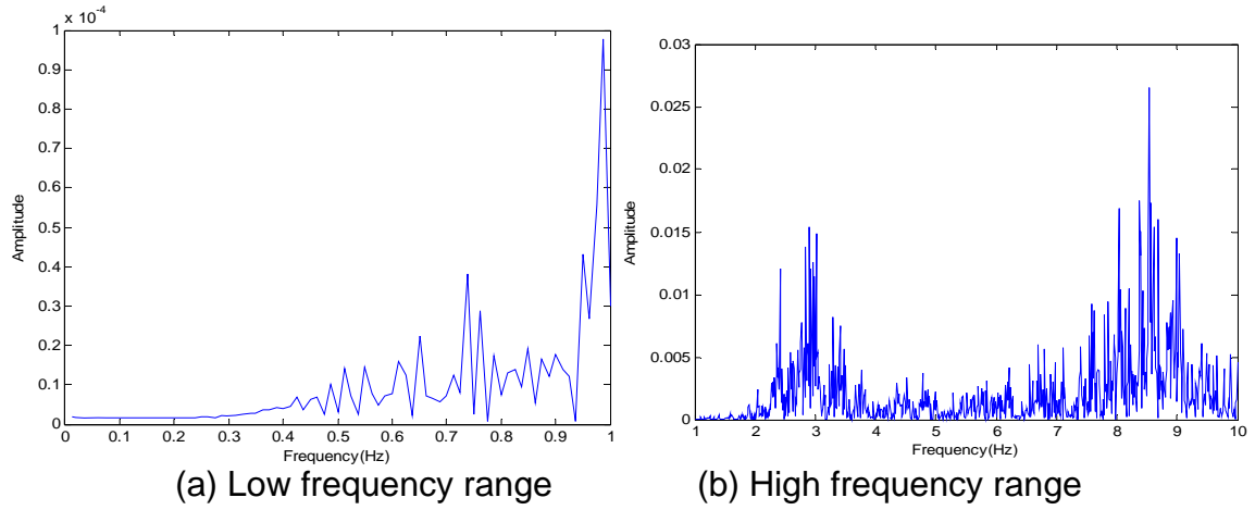
Figure 3.20 Fourier spectrum of acceleration at HNZ-P8
