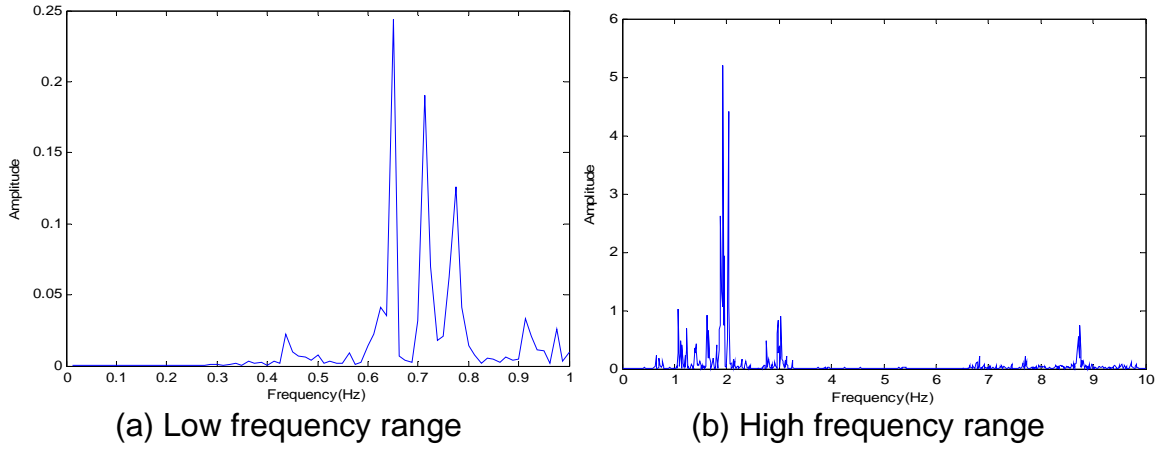
Figure 3.29 Fourier spectrum of acceleration at HNZ-R5
