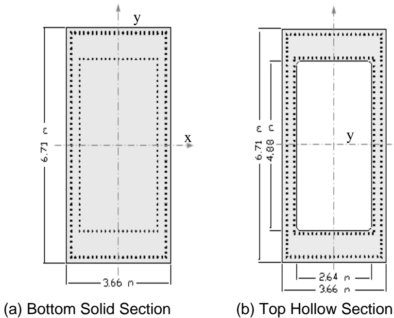
Figure 6.12 Cross sections of columns in towers
