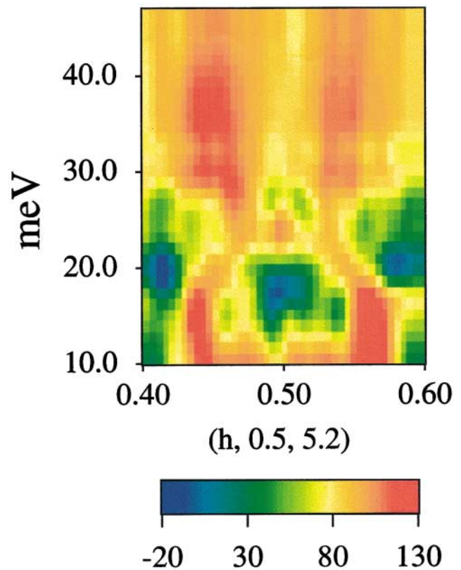
FIG. 3 (color). Magnetic scattering distribution for YBCO6.35 obtained by subtracting 100 K data from data taken at 10 K. The small resonance can be observed at (0.5, 0.5, 5.2) and 23 meV. The intense incommensurate scattering between 12 and 17 meV is at the right wave vector for charge and spin scattering to result from a striped phase.
