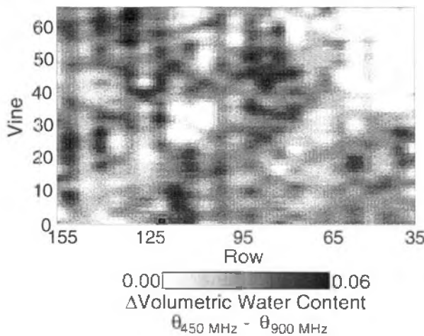
b) September 2001, \theta_{450} - \theta_{900} , \overline{\Delta\theta}_v = 0.029
