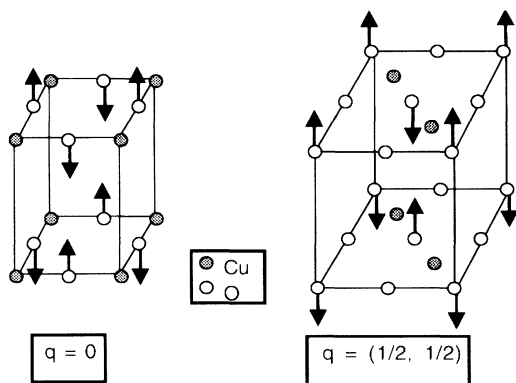
FIG. 2. Calculated eigenvectors of the 42.7 meV phonon for \mathbf{q} = 0 and \mathbf{q} = (\frac{1}{2}, \frac{1}{2}, 0) . Only one \text{CuO}_2 bilayer is shown. The arrows indicate the displacements of the in-plane oxygen ions. For clarity, smaller displacements of the Cu and Y ions are not indicated. In order to display the full symmetry of the mode, a \sqrt{2}a \times \sqrt{2}a cell is shown for \mathbf{q} = (\frac{1}{2}, \frac{1}{2}, 0) .
