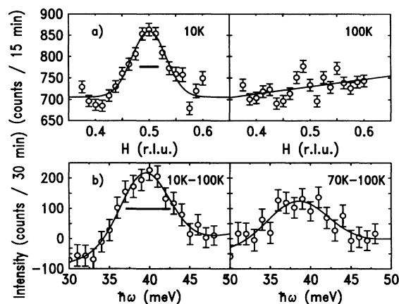
FIG. 4. (a) Constant-energy scans with \hbar\omega = 41 meV along (3H, H, 1.7) and (b) constant- \mathbf{Q} scans with \mathbf{Q} = (\frac{3}{2}, \frac{1}{2}, 1.7) . In (b) the difference between 10 K (70 K) and 100 K is plotted. The raw data also show a contribution of a phonon centered at \hbar\omega \sim 30 meV. The instrumental momentum and energy resolutions are indicated by bars. The solid lines are guides to the eye.
