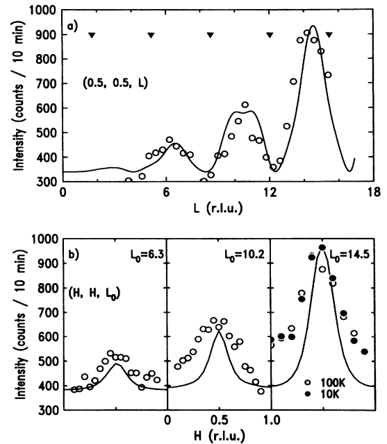
FIG. 1. Constant-energy scans with \hbar\omega = 41 meV along (a) \mathbf{Q} = (\frac{1}{2}, \frac{1}{2}, L) and (b) \mathbf{Q} = (H, H, L) with fixed L . The solid lines are predictions of a lattice dynamical calculation for scattering from the 42.7 meV oxygen vibration. Only the background and the overall scale were adjusted. The arrows in (a) indicate the maxima of \sin^2(\pi z_{\text{Cu}} L) [Eq. (2) in the text].
