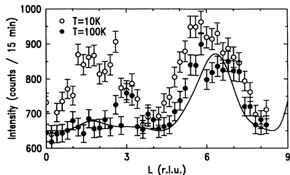
FIG. 3. Constant-energy scans with \hbar\omega = 41 meV along \mathbf{Q} = (\frac{3}{2}, \frac{1}{2}, L) in the normal and superconducting states. The solid line is the prediction of the lattice dynamical calculation for scattering from the 42.7 meV phonon.
