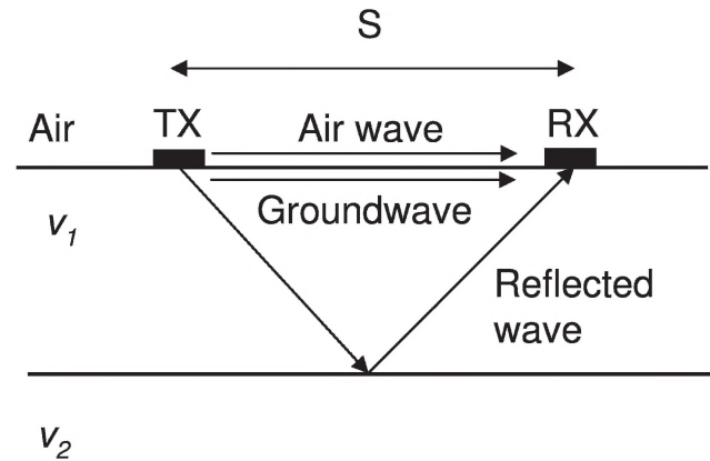
Figure 1. The GPR groundwave travels in the shallow subsurface between the transmitting antenna (TX) and receiving antenna (RX). S is the separation distance between the GPR antennas, while v_1 is the velocity of the uppermost soil layer.
