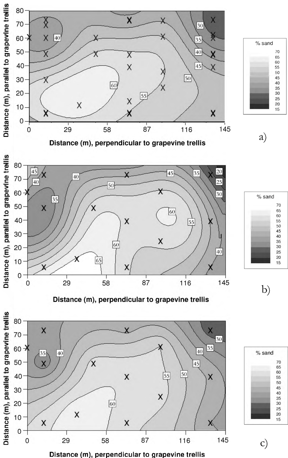
Figure 12. a) Contour map of the percent sand in the uppermost 20 cm developed using kriging of all CGSF measurements in rows without crop cover. b) Contour map of the percent sand developed using kriging of a subset of CGSF measurements in rows without crop cover. c) Contour map of the percent sand developed using co-kriging of a subset of CGSF measurements in rows without crop cover and volumetric water content estimates from 450 MHz GPR data acquired in Jan.
