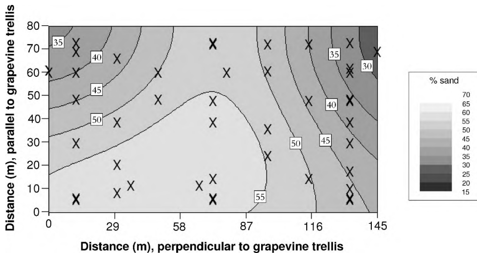
Figure 4. Contour map of soil sand fraction (% sand) in the uppermost 20 cm of the soil column across the site.
