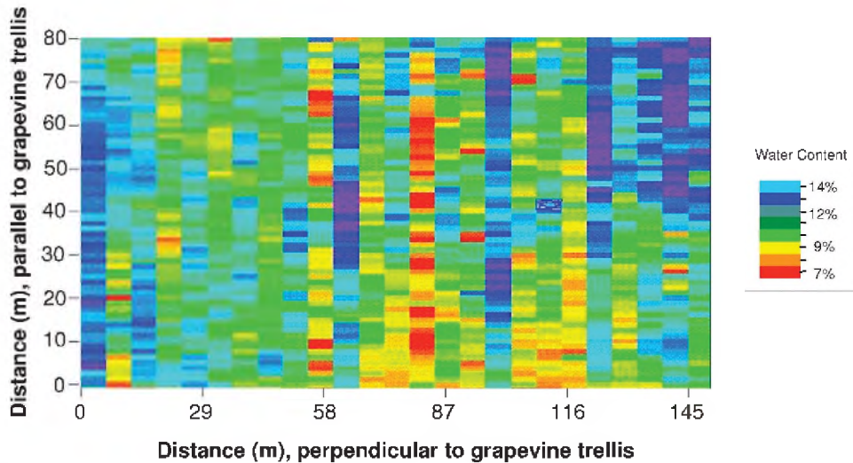
Figure 3. Water content estimates acquired over the three acre field site in Sept. 2001 using 900 MHz GPR groundwater data. Each vertical “stripe” corresponds to a GPR traverse, where a traverse parallel to the grapevine trellis was collected every 6 m with sampling every 10 cm along the traverse.
