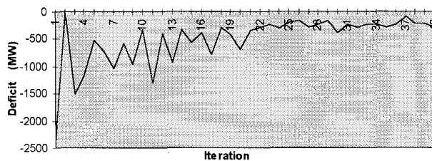
Fig. 3 Spinning reserve deficit vs. iteration
