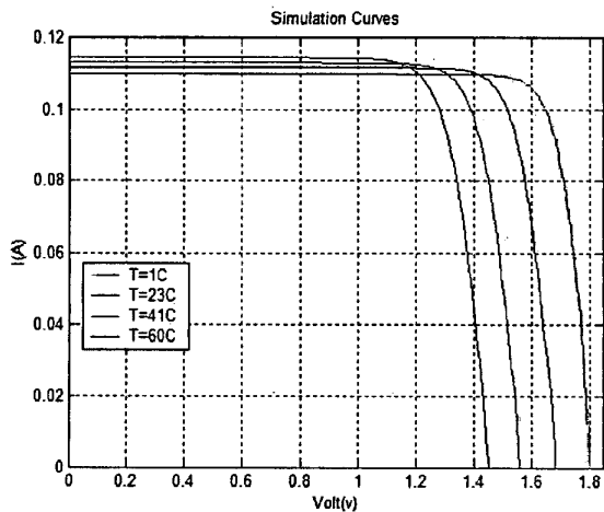
Fig. 4.1. Simulated I-V Curves
