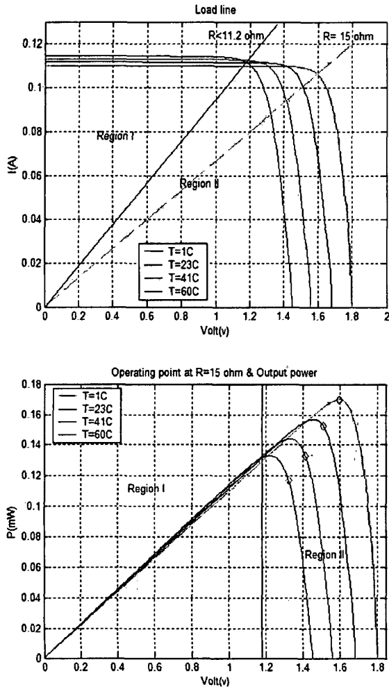
Fig. 4.4. Two loading regions and corresponding power curves
