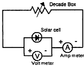
Fig. 3.2. Circuit for measuring solar cell characteristic
