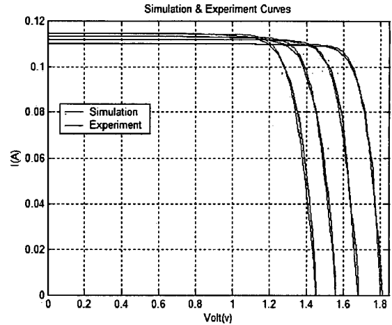
Fig. 4.2. Comparisons of Simulation and Experiment
