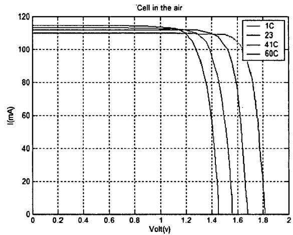
Fig. 3.3. I-V characteristic curve as a Function of Temperature
