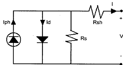
Fig. 2.2 Equivalent circuit of the solar cell
