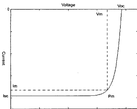
Fig. 2.3. Characteristic curve of the solar cell
