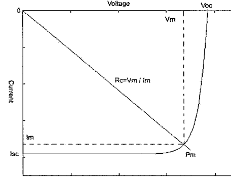
Fig. 2.4. Characteristic resistance load line
