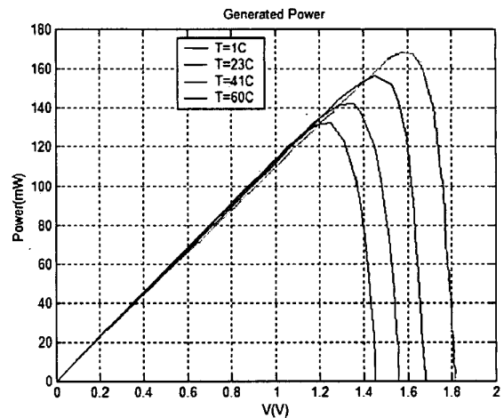
Fig. 3.4. Power output as a Function of Temperature
