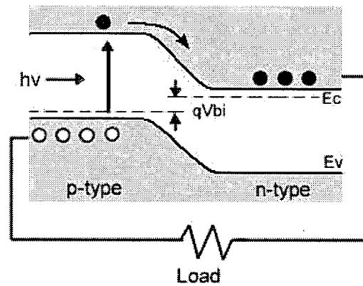
Fig. 2.1. Semiconductor p-n junction under illumination
