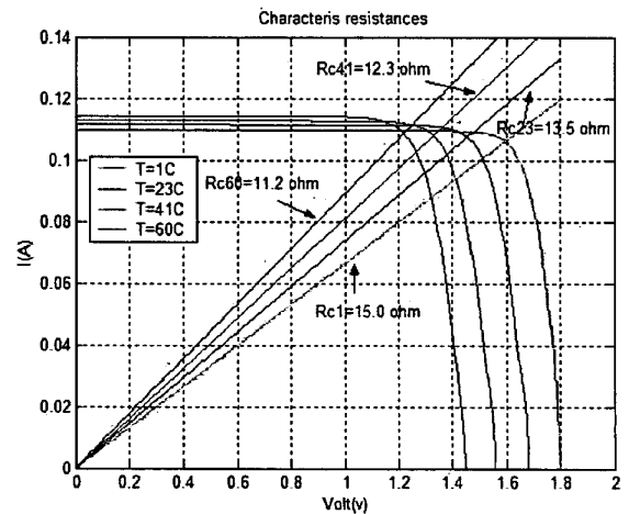
Fig. 4.3. Characteristic resistances at each temperature
