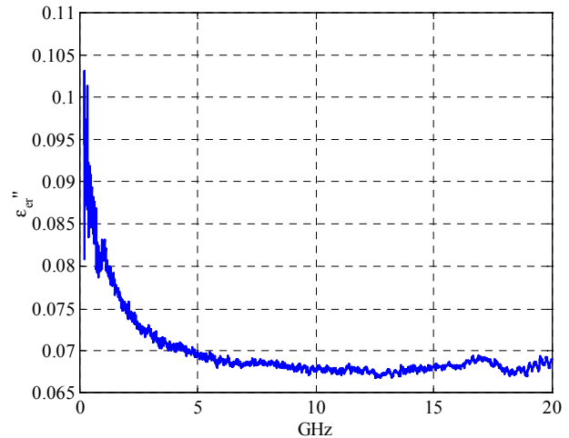
Figure 3. Characterized the imaginary part of the permittivity of the stripline including \sigma_e .
