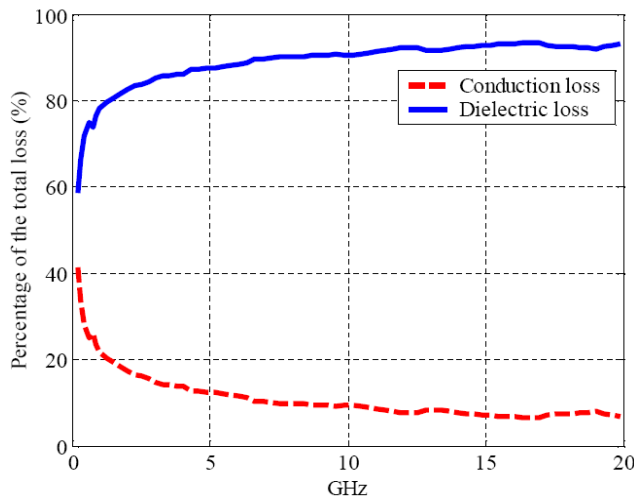
Figure 5. Quantified dielectric loss and conductor loss.
