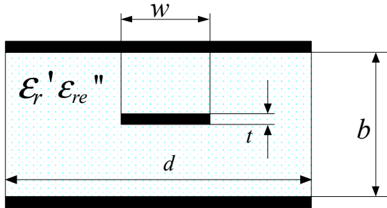
Figure 1. Cross-section of a stripline.
