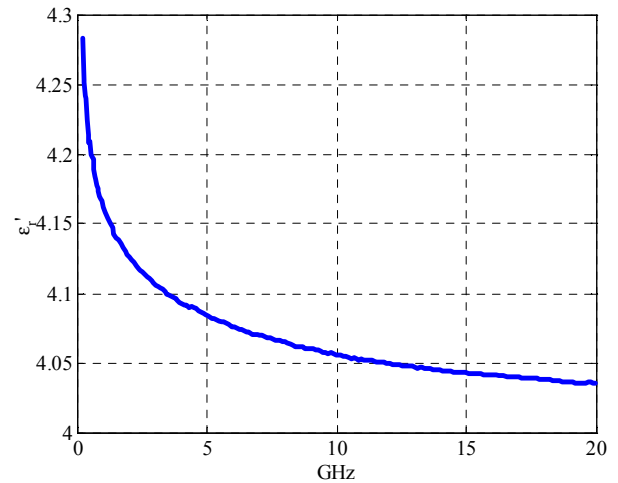
Figure 2. Characterized the real part of the permittivity of the stripline.
