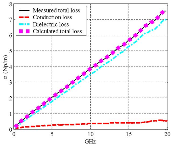
Figure 4. Calculated dielectric loss, conductor loss, and total loss as well as the measured total loss.
