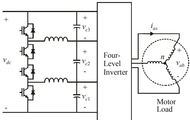
Figure 1. Proposed 4-level two-quadrant dc/dc converter.
