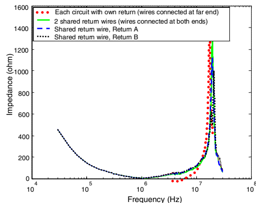
Figure 1. Measured impedance of power control module and harness connections.
