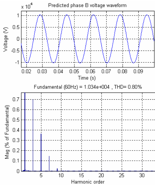
Fig. 13. Plot of phase B voltage predicted by ANN2
