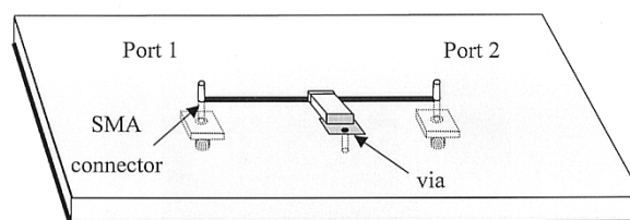
Fig. 3. Test board with a one-capacitor, low-pass filter.
