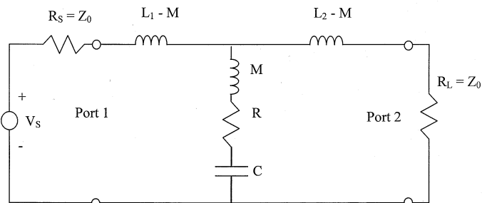
Fig. 1. Equivalent circuit of a low-pass filter.
