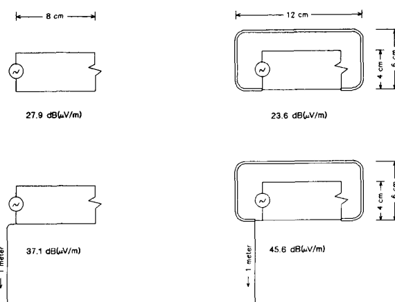
Fig. 17. Wire model of circuit with and without a shield.
