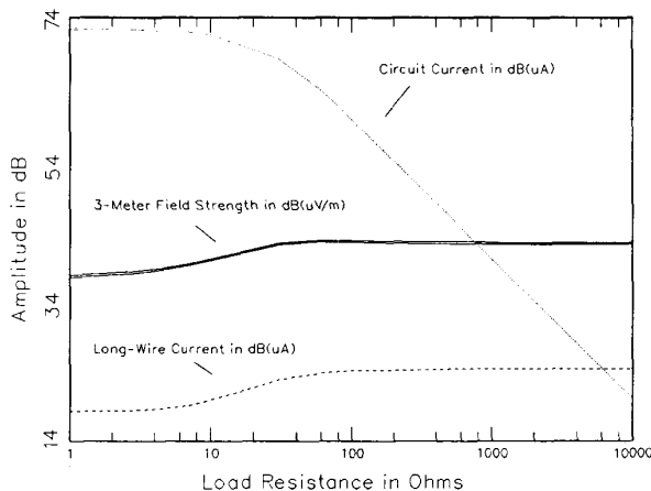
Fig. 4. Field strength and currents as a function of load resistance.
