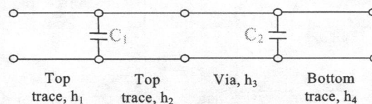
Figure 3. An equivalent circuit for the geometry shown in Fig. 1.
