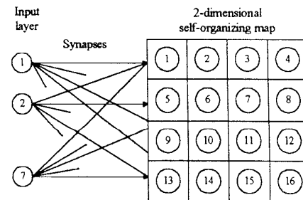
Fig. 4. The Kohonen neural network
