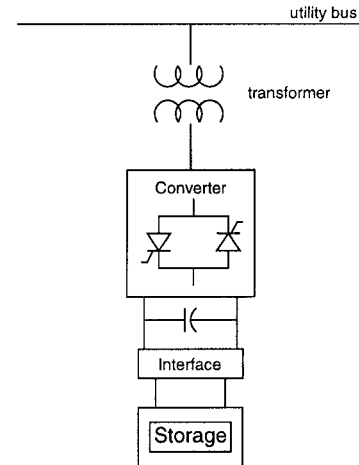
Figure 1 – Integrated StatCom with Energy Storage
