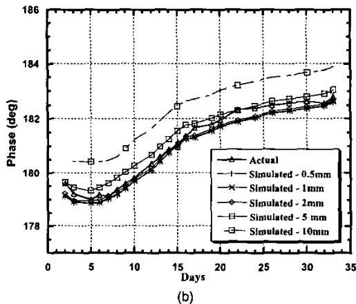
Fig. 2. Simulation results at 3 GHz, (a) magnitude and (b) phase.
