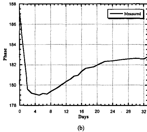
Fig. 1. Reflection properties at 3 GHz, (a) magnitude and (b) phase.
