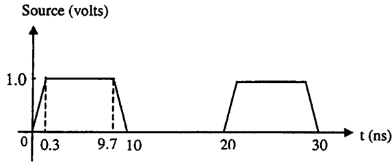
Figure 3. The input waveform at Point 1.
