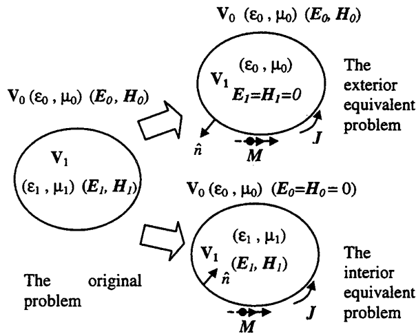
Figure 4. The original problem can be decomposed into the exterior equivalent and the interior equivalent problems.
