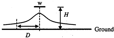
Figure 9. High-frequency current distribution under a trace.
