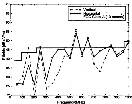
Figure 10. The maximum 10-meter electric field.
