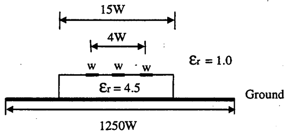
Figure 8. Cross-sectional view of the truncated problem.
