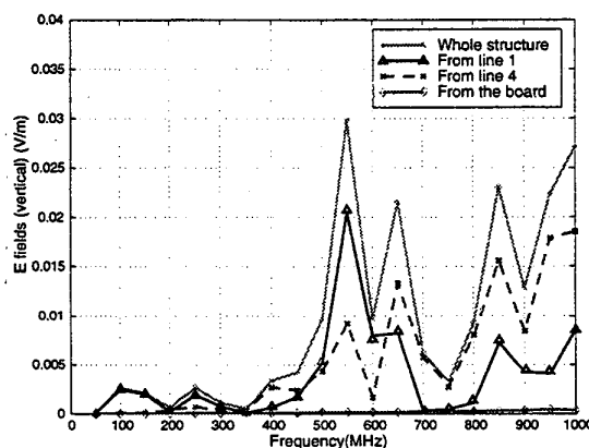
Figure 12. The maximum vertical electric field 10 meters from the board with a normalized source.
