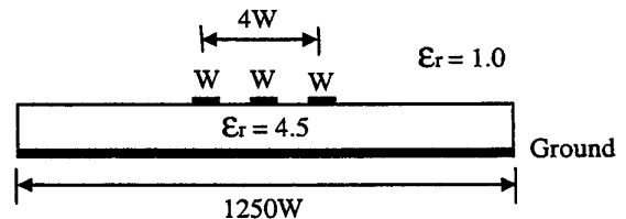
Figure 7. Cross-sectional view of the three coupled traces.
