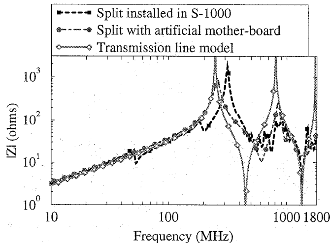
Figure 11. Comparison of the magnitude of the impedance for the transmission-line model, experimental data for the split groundplane installed in the S1000, and experimental data with the artificial mother-board.
