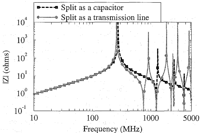
Figure 5. Comparison of the magnitude of the impedance for the split modeled as a capacitor and the split modeled as two parallel transmission lines.
