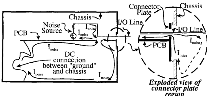
Figure 2. Schematic showing how noise coupled to an I/O line may radiate from a device. The schematic shows a split groundplane and depicts how noise currents may be conducted around the inside of the chassis, because of the relatively high impedance of the split.
