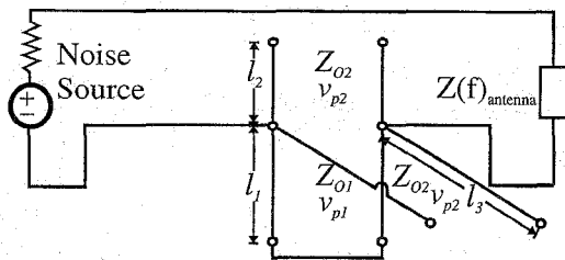
Figure 4. Circuit model depicting a noise source driving an I/O line over a split groundplane. L_{loop} and C_{split} have been replaced with transmission-line models.
