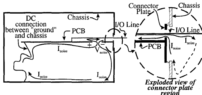
Figure 3. Schematic showing how a split groundplane may increase radiation if the power-bus is noisy with respect to the chassis.
