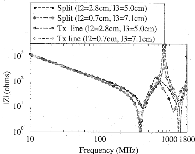
Figure 10. Comparison of the magnitude of the impedance for the transmission-line model and experimental data for the split groundplane not installed in the mother-board. The impedance was measured at two locations, l_2 = 2.8 \text{ cm} , l_3 = 5.0 \text{ cm} and l_2 = 0.7 \text{ cm} , l_3 = 7.1 \text{ cm} (see Figure 6).
