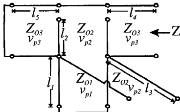
Figure 8. Transmission line model for measuring the impedance of the groundplane split with the test-board.
