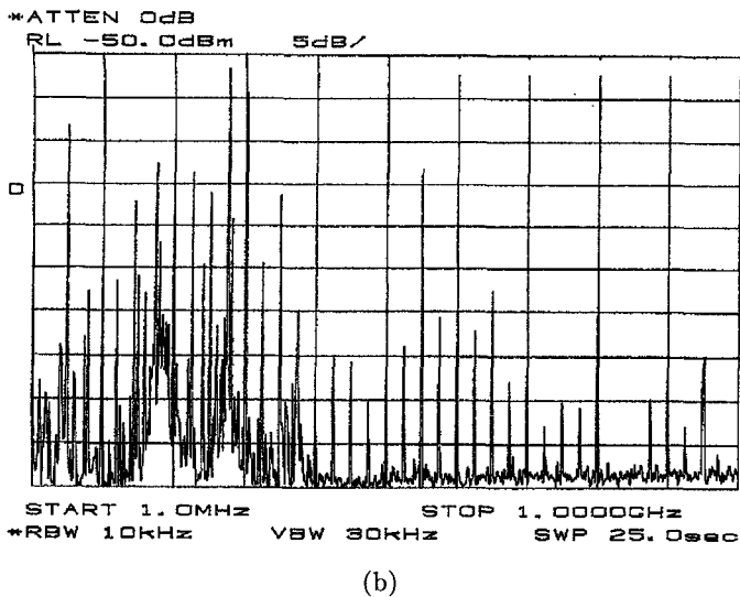
Figure 12. Radiated fields for the test-card installed in a S1000 with (a) the continuous groundplane test-card, and (b) the split groundplane test-card.
