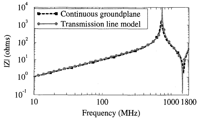
Figure 9. Comparison of the magnitude of the impedance for the transmission-line model and experimental data for the continuous groundplane test-board.
