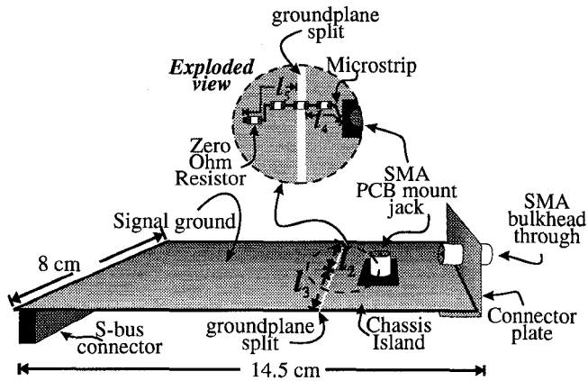
Figure 6. Test-board layout showing the basic setup for taking measurements. The exploded region shows how the center conductor of the SMA jack was routed over the trace to the signal ground using microstrip traces and zero ohm resistors. The lengths designated by l_2, l_3, l_4, and l_5 are the lengths of the transmission lines comprising the equivalent circuit model.
