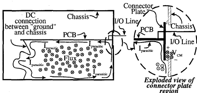
Figure 1. Depiction of how conducting loops and poor connector plate connectivity may result in radiated fields. The connector plate region is exploded to show detail.
