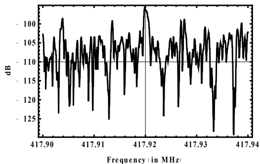
Figure 2a: Electromagnetic Emission with 1001 Observations
