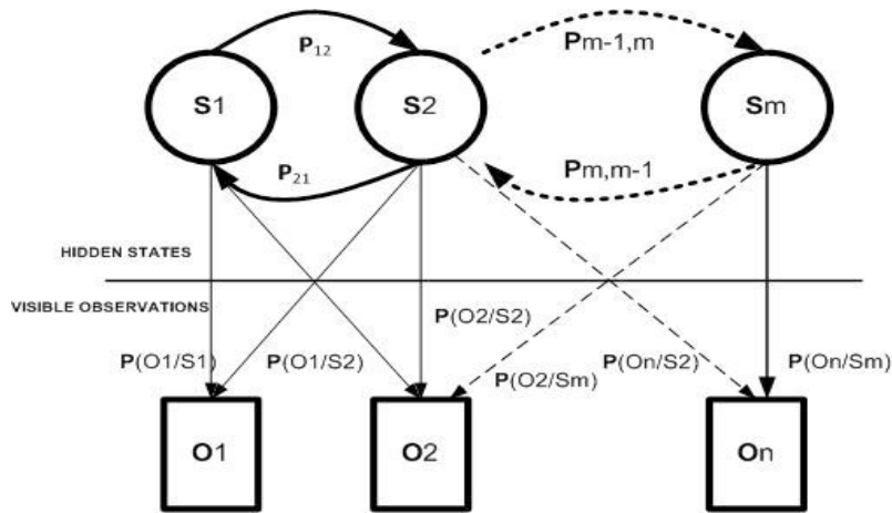
Figure 3: HMM Representation
