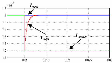
Fig. 11. L_{real} , L_{asmds} and L_{adjis} when L_{asmd} changes from 20 \mu\text{H} to 15 \mu\text{H} at 0.01 s.
