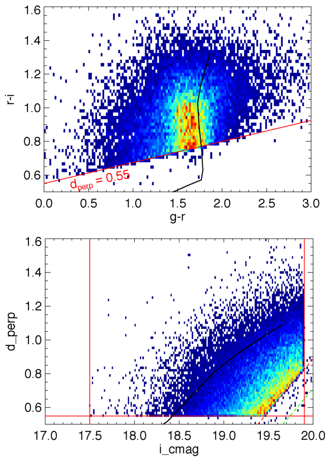
Figure 4. Both panels show density plots of CMASS galaxies; red corresponds to higher density and dark blue to lower density in an arbitrary normalizing and linear scale. The black thick line shows the passively evolving LRG model of Maraston et al. (2009). Top: redshift increases upwards, starting at z \simeq 0.4 at d_{\perp} = 0.55 . Bottom: the sliding cut in d_{\perp} with i -band magnitude, designed to select an approximately stellar-mass complete sample. Stellar mass increases with the perpendicular distance to the sliding cut, represented here by the red dashed line – see Maraston et al. (2013) for details. The green dashed line shows the sliding cut adopted for the CMASS SPARSE sample (see Section 3.4). Vertical solid lines show the magnitude limits. On both panels, the small fraction of targets that lie outside of the selection cut are due to differences in the targeting and final photometry, see Section 2. Only chunks greater than 6 are shown.
