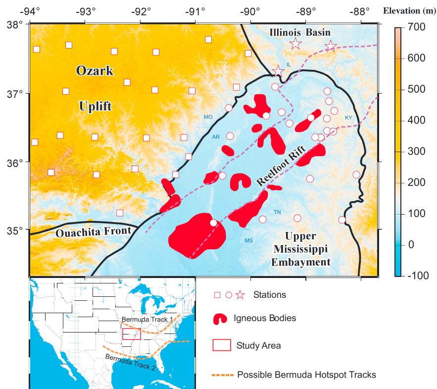
Figure 1. Topographic map showing boundaries of major tectonic features (black lines), igneous bodies (red areas) [Hildenbrand et al. , 1996], and broadband seismic stations used in the study. Stations represented by squares, circles, and stars are located in the Ozark Uplift, Upper Mississippi Embayment, and the Illinois Basin, respectively. The area between the purple dashed lines is the Reelfoot Rift, in which the NMSZ is located. The inset in the lower left corner displays the map of the contiguous United States showing the location of study area (red rectangle) and proposed possible Bermuda hotspot tracks (orange dash lines) [Pollitz and Mooney, 2014].
