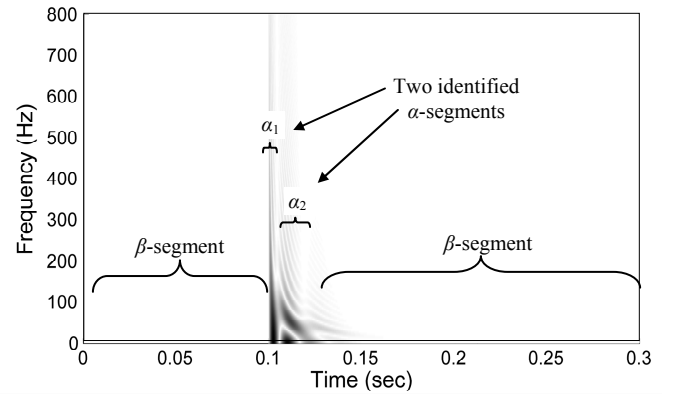
Fig. 2. Wigner-Ville time-frequency decomposition of e_0(k) .
