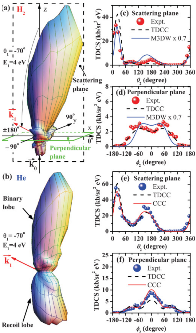
FIG. 1. (Color online) 3DCS for H_2 (three top diagrams) and He (three bottom diagrams) as a function of the emission angle of an electron with kinetic energy E_2 = 12 eV. The emission angle of the other electron ( E_1 = 4 eV) is fixed to \theta_1 = -70^\circ : (a) and (b) Experimental 3D-cross sections for H_2 and He, respectively: (c) and (d) Cross section cuts for H_2 in the scattering and perpendicular planes, respectively. \phi_2 is the emission angle in the perpendicular plane with respect to the x -axis. The experimental data are given by full circles. (e) and (f) same as (c) and (d) but for He.
