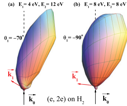
FIG. 5. (Color online) TDCC results for the 3DCS of the H_2 target covering 4\pi solid angle of electron emission. (a) E_1 = 4 eV, E_2 = 12 eV, \theta_1 = -70^\circ . (b) E_1 = E_2 = 8 eV, \theta_1 = -90^\circ .
