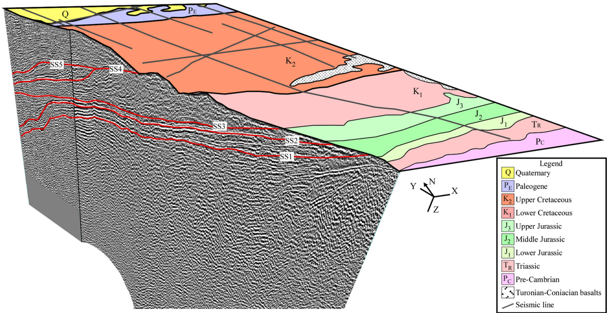
Fig. 5. Three-dimensional diagram displaying the methodology used to establish the chronology of seismic surfaces using the geological map of the Mahajanga Basin. See Figure 2 for location of seismic line. Seismic line courtesy of OMNIS and CGG MCNV (GeoSpec). Geological map is highly modified from Roig et al. (2012). Diagram not drawn to scale. See Figs. 2 and 4 for scale.
