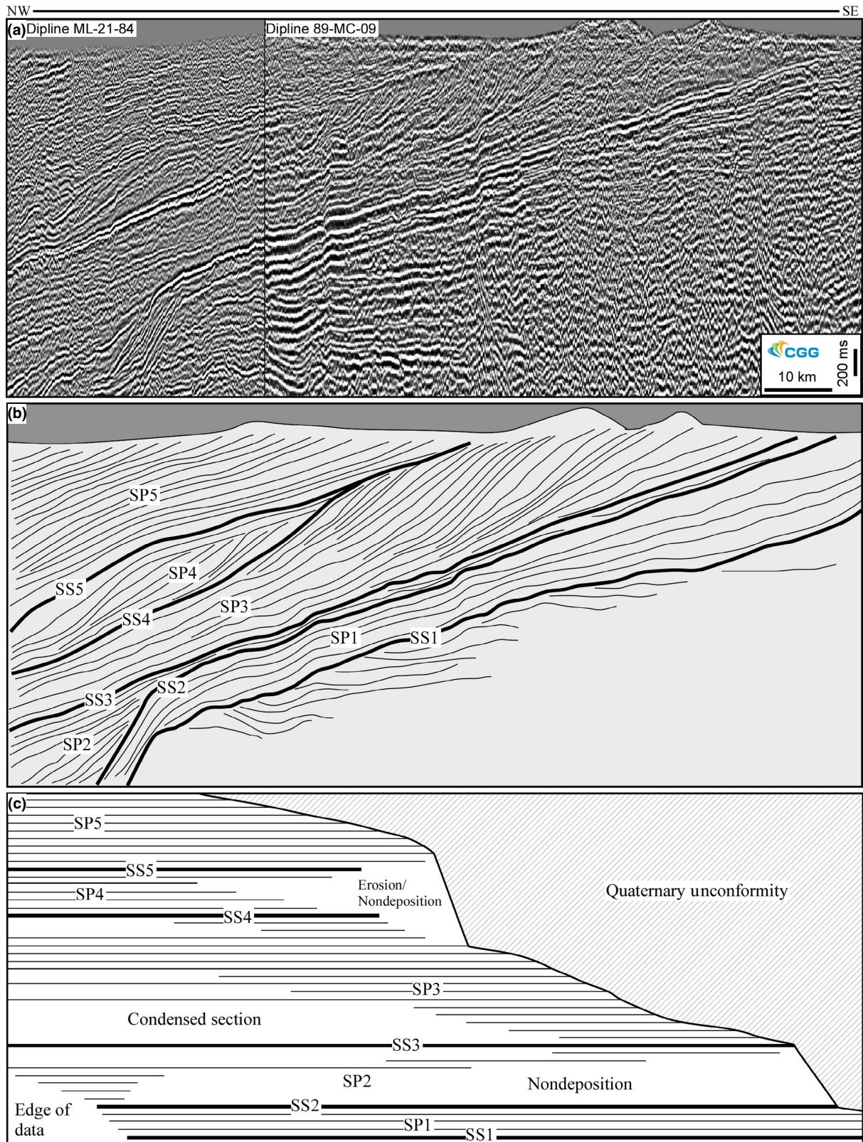
Fig. 4. (a) Uninterpreted seismic line from the Mahajanga Basin. (b) Interpreted schematic diagram of seismic line. Notice the exposure of sloping segments and topsets of clinoforms onshore Madagascar. Seismic surfaces and packages are described in the text. (c) Chronostratigraphic interpretation (Wheeler diagram) of seismic profile in 4a. See text for details. See Figure 2 for location of seismic line. Seismic line courtesy of OMNIS and CGG MCNV (GeoSpec).
