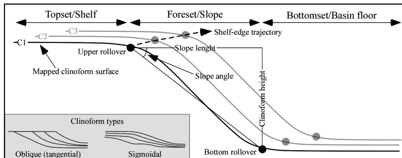
Fig. 6. Simplified cross-sectional schematic profile of a clinoform highlighting depositional provinces, geometries calculated in this study, and points of significant change in slope (rollover points). Modified from Helland-Hansen & Hampson (2009). Grey box contains a schematic profile of the two types of clinoforms recognized in this study. Modified from Mitchum et al. (1977).
