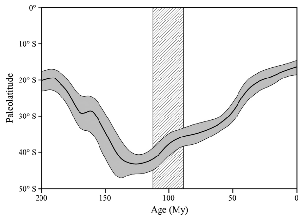
Fig. 11. Paleolatitude migration of Madagascar from 200 Ma to its present position at ca. 16.4° S. Notice the slow northward migration of Madagascar from ca. 130 Ma to present. Grey envelope is the 95% confidence interval on paleolatitude and hatched area highlights the approximate time during which progradation of the siliciclastic margin occurred. Paleolatitude from van Hinsbergen et al. (2015).
