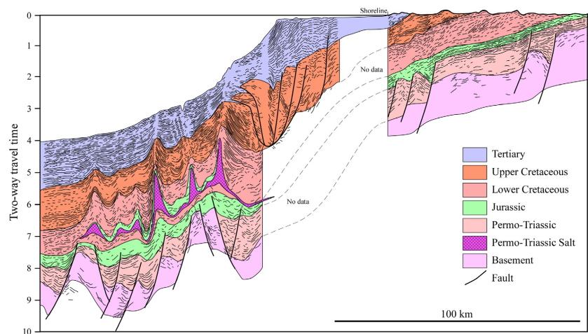
Fig. 8. Regional interpreted geoseismic transect across the northern part of the Mahajanga Basin with a vertical exaggeration of 4 km sec -1 . Modern shelf is a poor seismic data area. See Figure 2 for location of seismic line. Geoseismic transect provided by G. Tari. Modified from Tari et al. (2004).
