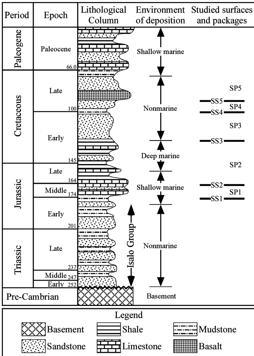
Fig. 3. Highly simplified stratigraphy and lithological column from Mahajanga Basin, NW Madagascar. Lithological column modified and simplified from Besairie (1972). Absolute ages at epoch boundaries from Gradstein et al. (2004). See Figure 4 and text for details on seismic surfaces and packages.
