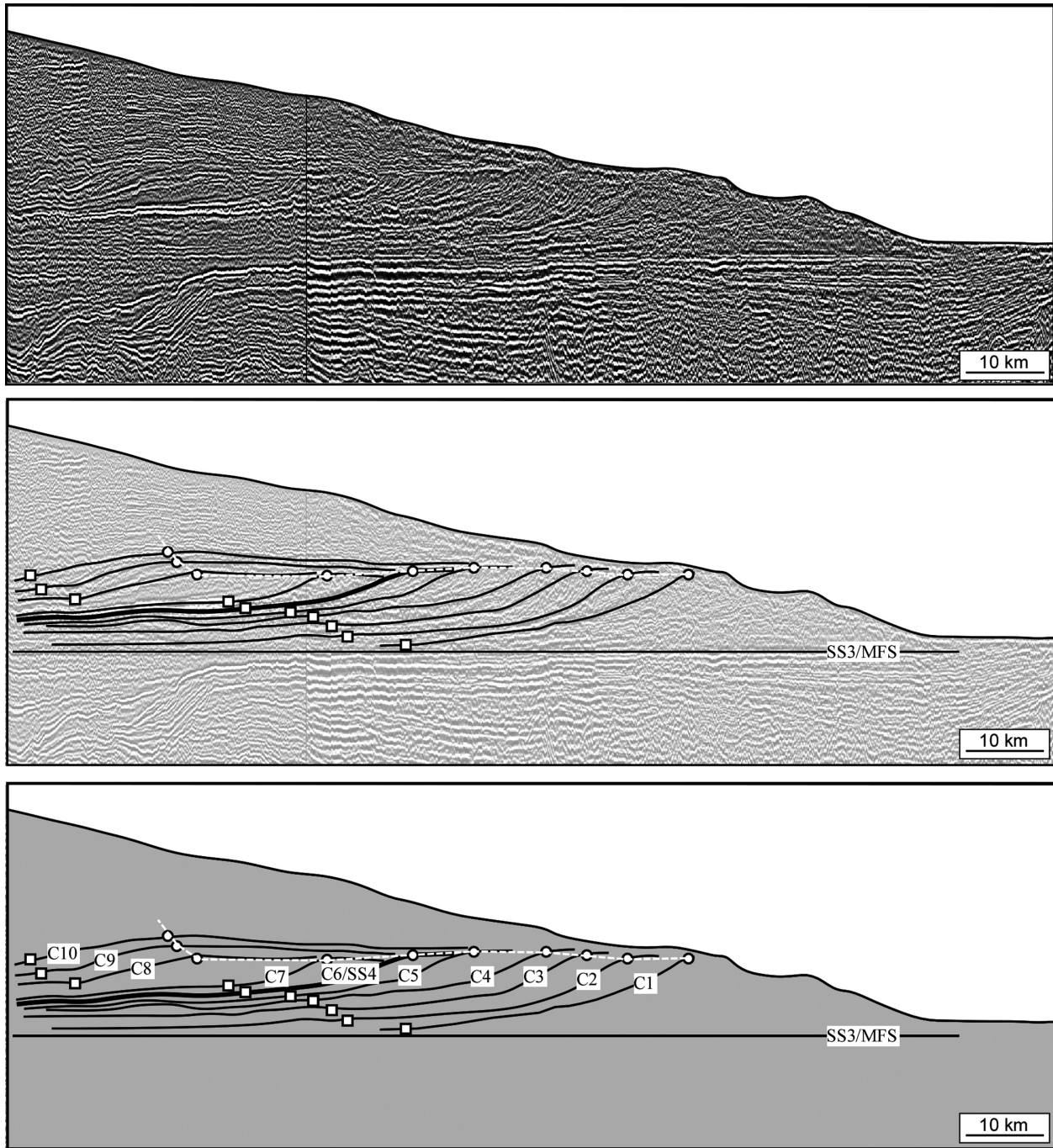
Fig. 9. Uninterpreted, interpreted and schematic diagram of clinoforms interpreted in this study. See Fig. 2 for line location. Seismic line is flattened on the maximum flooding surface (SS3). Notice the flat trajectory of C1 through C6, the change to a downward-directed trajectory from C6 to C8 and the change to an ascending trajectory from C8 to C10. Black and white circles mark the interpreted topset to foreset transition; white dashed line is the overall trajectory of the shelf edge. Black and white squares mark the interpreted foreset to bottomset transition.
