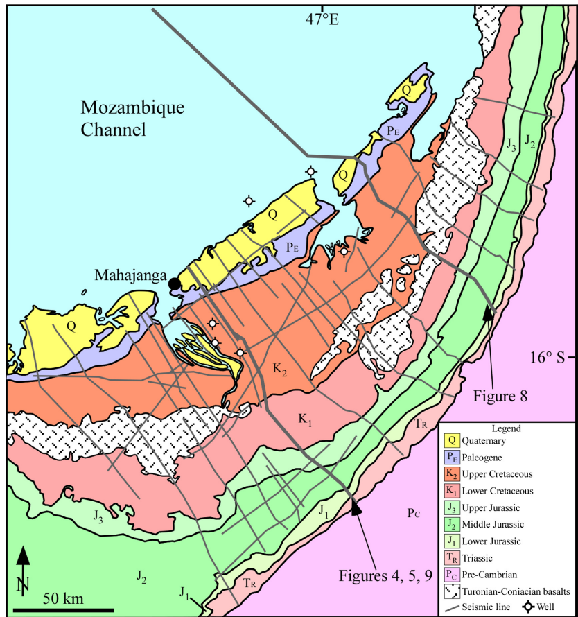
Fig. 2. Geological map of the Mahajanga Basin, northwest Madagascar with location of 2D seismic profiles used in this study. Geological map is highly modified from Roig et al. (2012). See Figure 1 for location of study area.
