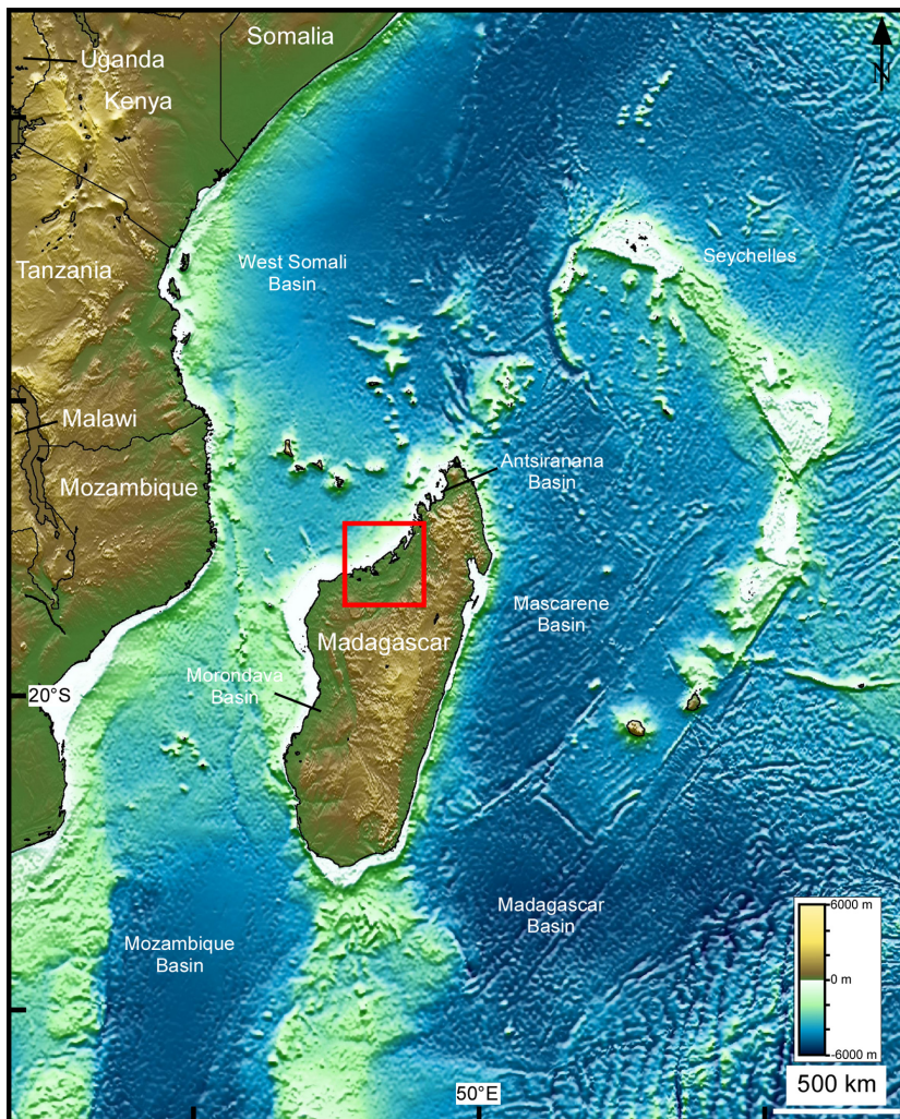
Fig. 1. Topographic relief map of eastern Africa with the location of major basins. Red box highlights the location of the study area within the Mahajanga Basin in northwest Madagascar.
