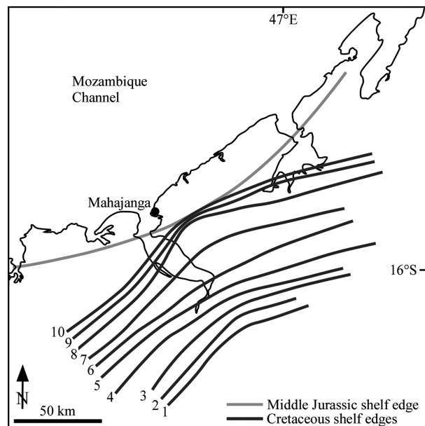
Fig. 7. Map of the Mahajanga Basin with the interpreted Middle Jurassic and Albian–Turonian shelf edges. The Middle Jurassic shelf edge is characterized by a westward facing convex morphology, while the prograding Albian–Turonian shelf edges are concave. Shelf-edge numbers correspond to the same numbered clinofolds in Fig. 9.
