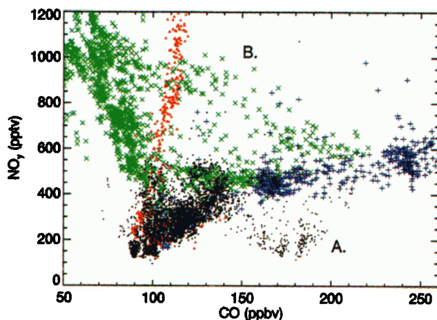
Figure 2. Observed NO y versus CO concentrations for altitudes between 8 and 12.5 km over the central United States (Figure 1). Each point is a 10-second average. Four populations are highlighted. The green crosses represent stratospheric data (N 2 O<310 ppbv and O 3 >100 ppbv). The blue pluses represent the flight of May 2 (strong convective influence), and the red triangles represent the flight of May 8 (strong lightning influence). The remaining data (black dots) are viewed as representing the upper tropospheric background. Fresh aircraft plume observations (CO 2 >368 ppmv and NO>300 pptv) have been excluded from this figure. Populations "A" and "B" are discussed in the text.
