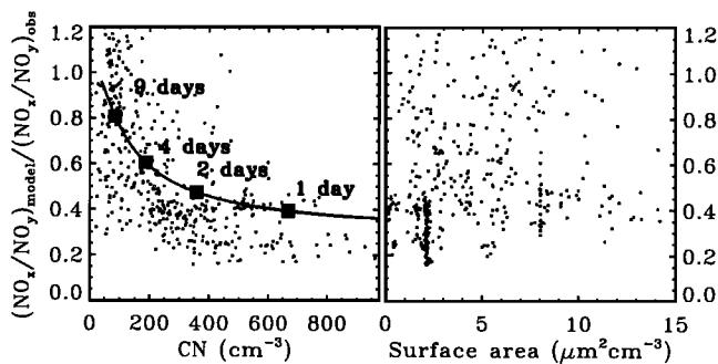
Figure 5. Left panel: Departure of the \text{NO}_x/\text{NO}_y concentration ratio from chemical steady state (model-calculated steady state \text{NO}_x/\text{NO}_y divided by the observed \text{NO}_x/\text{NO}_y ) as a function of condensation nuclei (CN) number concentration. The data are from all the SUCCESS flights over the central United States (Figure 1) above 8-km altitude. Observations in clouds (aerosol surface area > 20 \mu\text{m}^2/\text{cm}^3 ) and aircraft exhaust plumes have been excluded. CN is used as a proxy for the time elapsed since the last convective event. The solid curve shows results from a time-dependent model calculation of the \text{NO}_x/\text{NO}_y ratio where the time coordinate is derived from the CN concentration (see text). Right panel: Same as left panel, but as a function of aerosol surface area.
