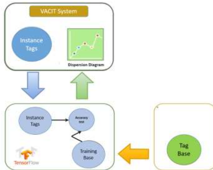
Figure 5. Machine Learning Module - Label Matching Level. Source: own.
