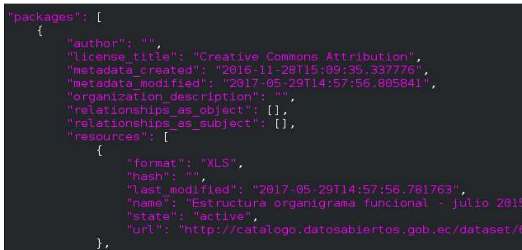
Figure 12. JSON segment with the metadata of a Ckan instance. Source: own.
