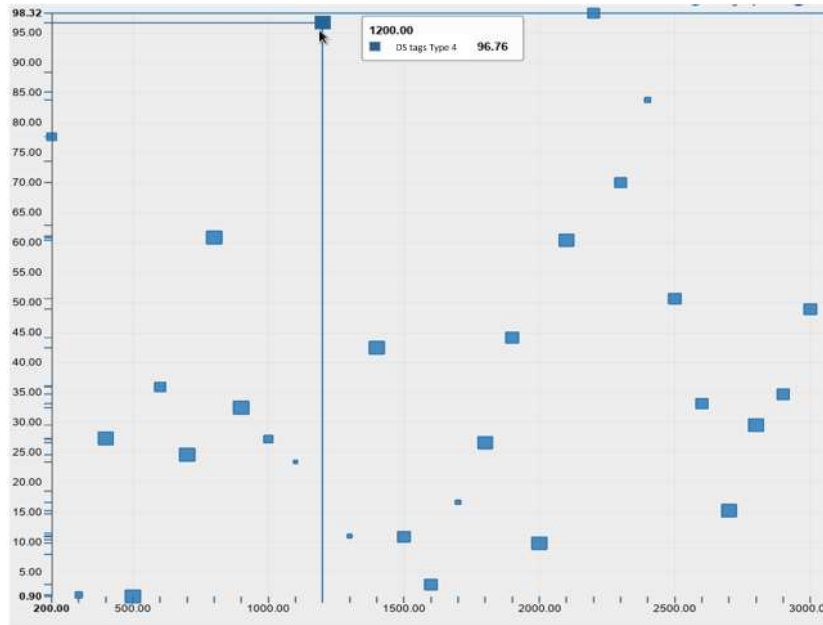
Figure 10. Conformance level of the domain labels of each dataset belonging to a CKAN instance. Source: own.
