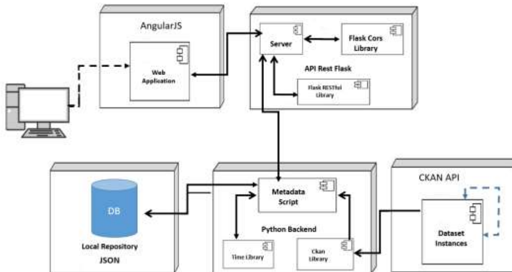
Figure 6. Architecture of the VACIT Tool. Source: own.
