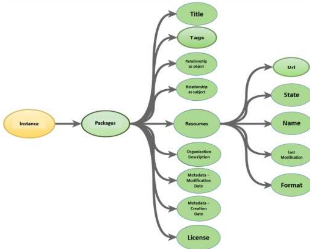
Figure 4. Dataset structure of a CKAN Instance. Source: own.
