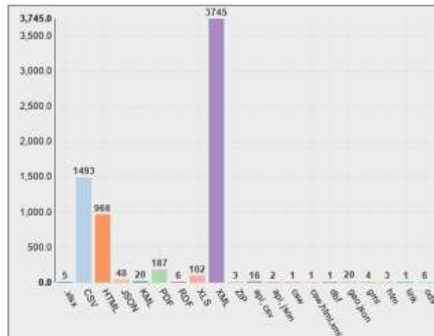
Figure 8. "Resource Format" Query in an instance. Source: own.
