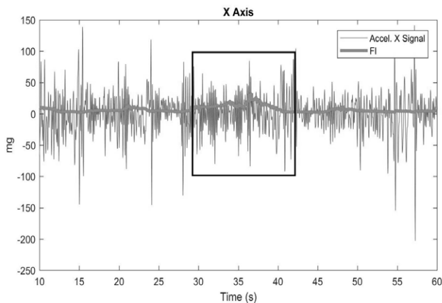
Figure 6. Simulated Parkinsonian gait signal together with the correspondence of Freeze Index using mobile windows for a subject. The black line indicates the period during which a freezing episode was simulated.
