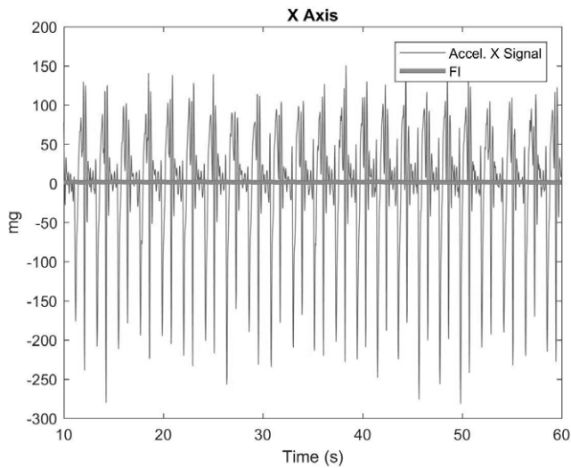
Figure 5. Normal gait signal along with Freeze Index correlation at instants of time using mobile Windows for a subject.
