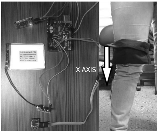
Figure 2. Wearable Device for FOG detection, image taken from a test subject to detect FOG. White arrow points out the X-axis.
