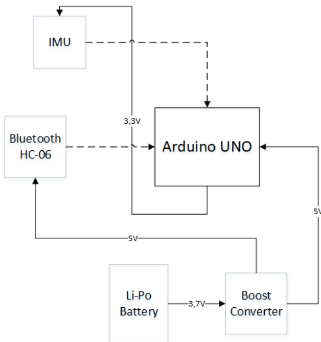
Figure 1. Connections of a wearable device for FOG detection.
