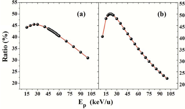
FIG. 3. (Color online) Theoretical PWBA TCS ratios of cusp-shaped electrons to the total electrons ejected in the single ionization of Ar and Ar + . (a) Theoretical results for He + ionizing Ar + ; (b) theoretical results for He 2+ ionizing Ar. Lines are a guide for the eyes.
