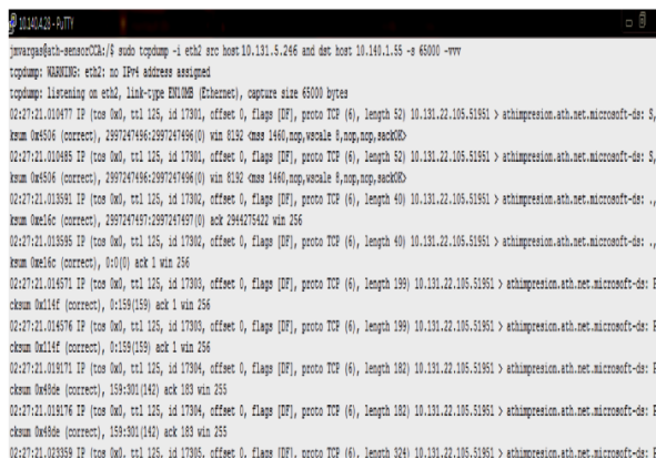
Figure 5: Traffic capture.
