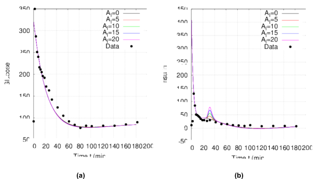
Figure 3: Variation of the glucose a) and insulin b) levels, based on time for different exogenous glucose quantities. The experimental data were reported and taken from [6].
