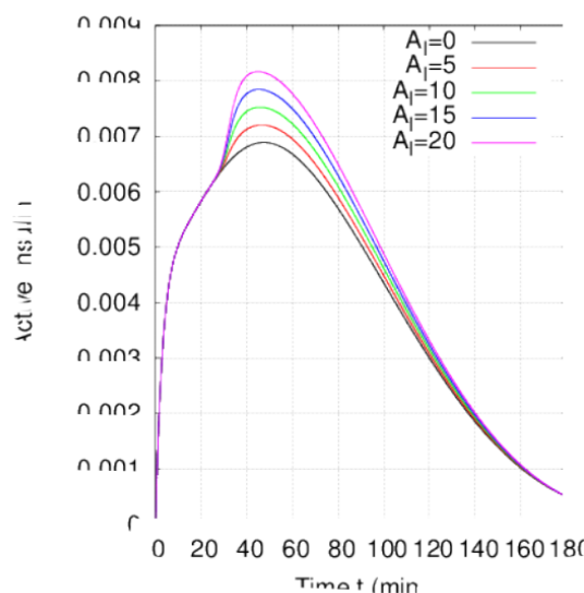
Figure 4: Variation of the active insulin levels based on time for different exogenous insulin quantities.
