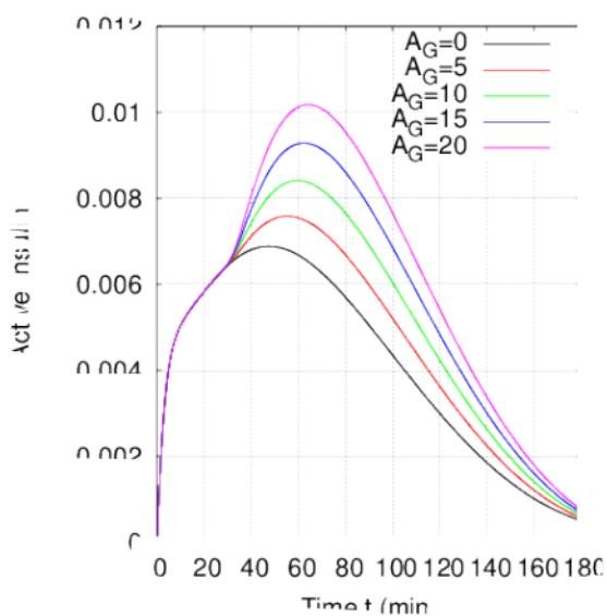
Figure 2: Variation of the active insulin levels based on time for different exogenous glucose quantities.
