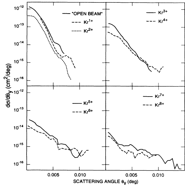
FIG. 10. Differential cross section and projection of angular distribution in the x - y plane for 10-MeV C^{6+} ions in coincidence with Kr^{q+} . "Open beam" depicts the beam profile not altered by target interactions.
