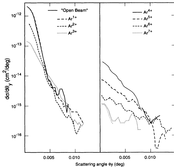
FIG. 9. Differential cross section and projection of angular distribution in the x - y plane for 10-MeV C^{6+} ions in coincidence with Ar^{q+} . "Open beam" depicts the beam profile not altered by target interactions.
