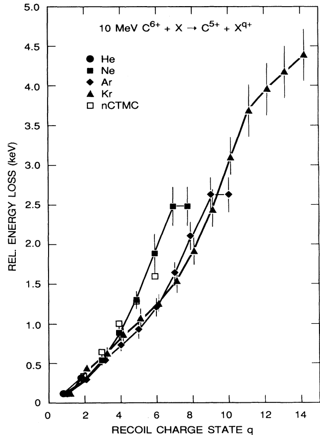
FIG. 11. Relative projectile energy loss for 10-MeV C^{6+} capturing one electron and multiply ionizing He, Ne, Ar, and Kr. The nCTMC calculations were done by Olson [26]. Only systematic error bars are shown. Statistical errors are negligible.
