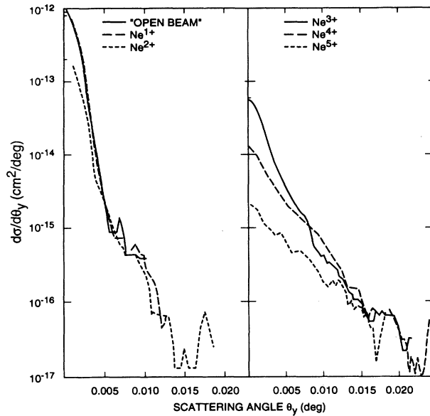
FIG. 8. Differential cross section and projection of angular distribution in the x - y plane for 10-MeV C^{6+} ions in coincidence with Ne^{q+} . "Open beam" depicts the beam profile not altered by target interactions.
