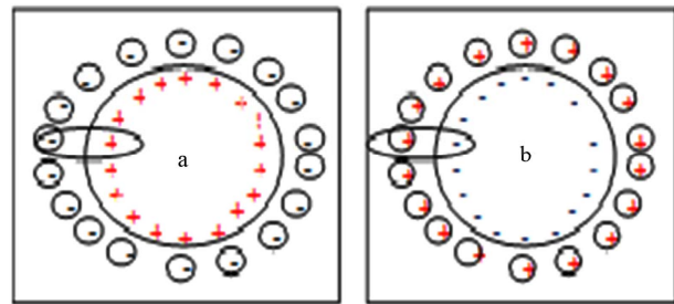
Figure 6. Matter-antimatter unification.
