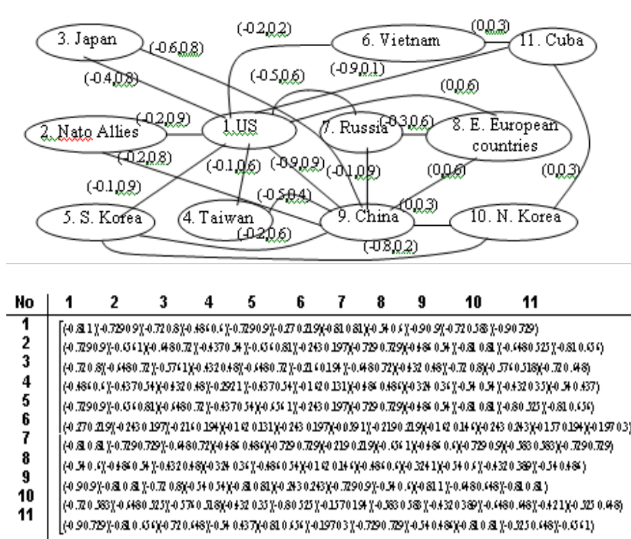
Figure 11. A bipolar cognitive map and its \oplus - \otimes transitive equilibrium relation.
