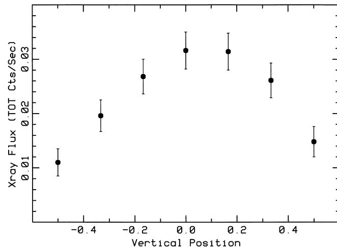
FIG. 4.—LSC emission fitted to map 2 for pillbox models with central planes offset from the Galaxy. Vertical position is expressed in terms of the thickness of the pillbox. The error bars are statistical only and are highly correlated. The units are the same as in Fig. 3.
