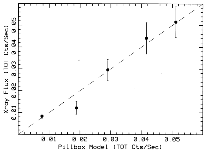
FIG. 6.—Average 2–10 keV flux of map 2 binned according to level of emission predicted from the pillbox model. The predicted emission is taken from Table 1, and the map is corrected for all fitted large-scale structure except for LSC emission. The error bars are statistical only. The units are the same as in Fig. 3.
