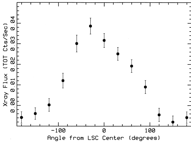
FIG. 3.—LSC emission fitted to map 2 for pillbox models lying in the supergalactic plane with centers rotated by angles in steps of 30^\circ from the nominal center of the LSC in Virgo. The error bars are statistical only and are highly correlated. The units are TOT counts s^{-1} ( 4.5 \text{ deg}^2)^{-1} \approx 1.54 \times 10^{-8} \text{ ergs s}^{-1} \text{ cm}^{-2} \text{ sr}^{-1} .
