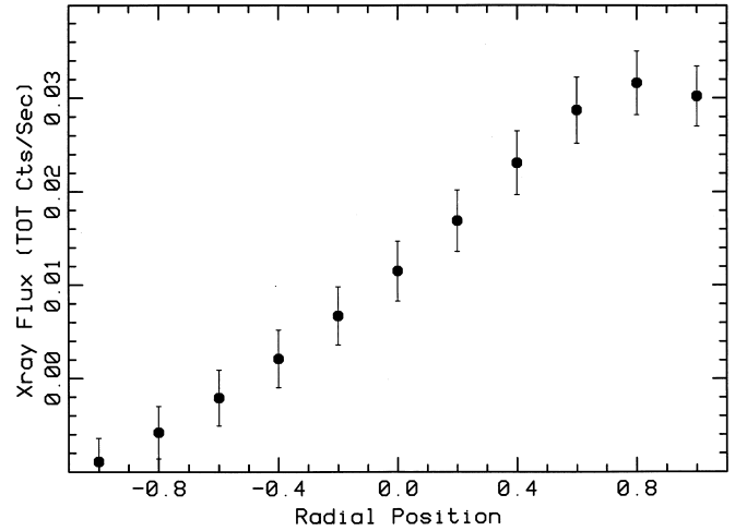
FIG. 5.—LSC emission fitted to map 2 for pillbox models with centers displaced from the Galaxy. Radial position is expressed in units of the supercluster radius. The nominal value is 0.8. Negative values indicate models with centers in the direction opposite Virgo. The error bars are statistical only and are highly correlated. The units are the same as in Fig. 3.
