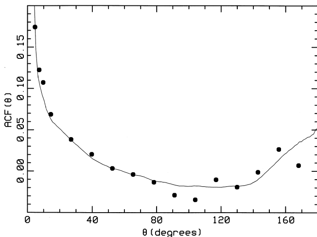
FIG. 7.—Autocorrelation function (normalized to unity) of map 2. For \theta > 10^\circ the data are binned in 13^\circ bins to reduce scatter. The solid curve is the ACF for the model including all fitted large-scale structure plus the fit of Fig. 2 for the small-scale ( < 10^\circ ) structure.
