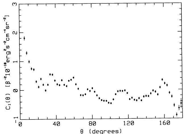
FIG. 1.—Autocorrelation function of the HEAO 1 A-2 X-ray map. \beta is a dimensionless parameter that depends on the spectrum. For a 10 keV bremsstrahlung spectrum, \beta = 1 . Error bars represent shot noise.
