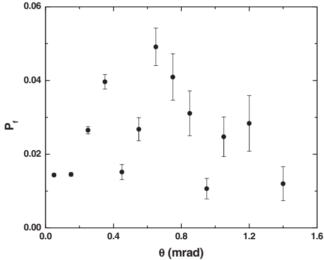
FIG. 6. Ratios P_f between the measured DDCS for proton fragment and \text{H}_2^+ formation as a function of scattering angle for \varepsilon = 27 eV.
