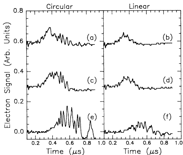
FIG. 6. Time-resolved field-ionization signal for both circularly and linearly polarized light with a peak ac Stark shift of approximately 600 \text{ cm}^{-1} . The lowest state shown is the n = 14 Rydberg state. (a) and (b) a tuning of 400 \text{ cm}^{-1} above the ionization limit, (c) and (d) a tuning of 200 \text{ cm}^{-1} above the ionization limit, and (e) and (f) a tuning to the ionization limit. For all of the tunings the residual Rydberg population is smaller for the linearly polarized case indicating that these Rydberg states are more easily ionized.
