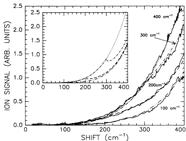
FIG. 4. Total ionization is shown vs the ac Stark shift produced by the peak of the laser pulse for laser tunings of 400, 300, 200 and 100 \text{cm}^{-1} above the four-photon ionization limit for circularly polarized light. Also shown are calculated spectra that include spatial averaging. The relative size of the four- and five-photon ionization cross sections was chosen to best fit the data. The inset shows the calculation without spatial averaging.
