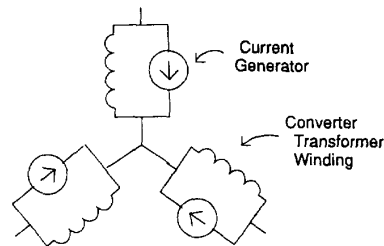
Figure 2: Separate Current Generators Used with Each Winding
