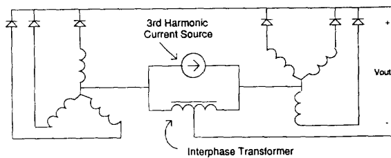
Figure 1: Duplex 6-Phase Rectifier with Third Harmonic Current Generator
