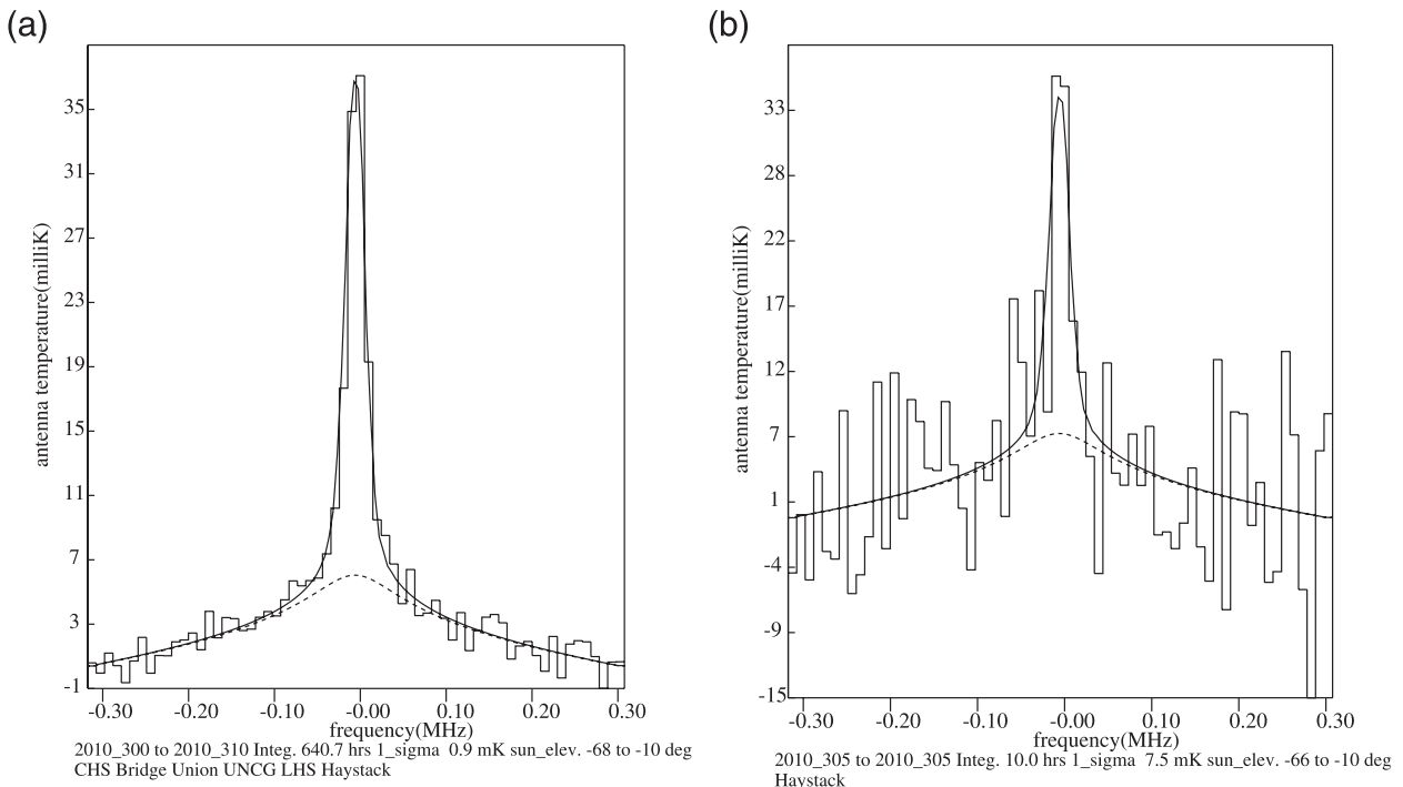
FIG. 2. (a) Spectrum of nighttime observations from all six sites from 27 Oct to 6 Nov 2010. The solid curve is the model fit to the data. The dashed curve and the difference between the solid and the dashed curves are the portions of the model for the ozone below and above 80 km, respectively. The two-component model fit to this data results in a peak volume mixing ratio of 14 ppmv of the assumed Gaussian profile for the ozone above 80 km. (b) Spectrum from a single night, 1 Nov 2010, at the Haystack site.
