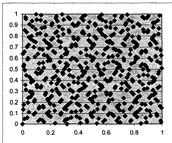
Figure 6: Same as Figure 5 with a Leap of 1024.
