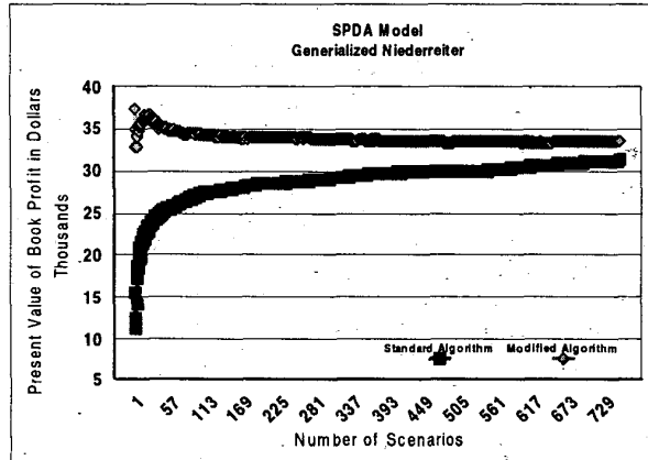
Figure 8: Niederreiter with and without Leaping
