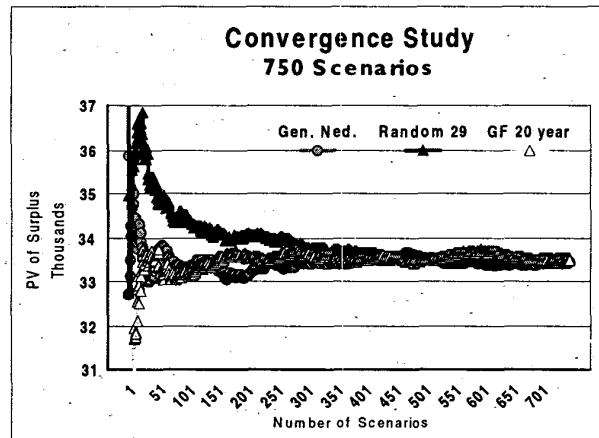
Figure 10: Comparing against Random Number Generation.
