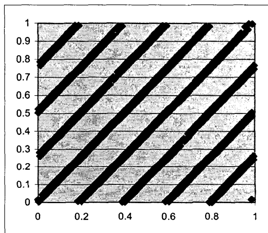
Figure 7: Same as Figure 2 with Leap of 251.
