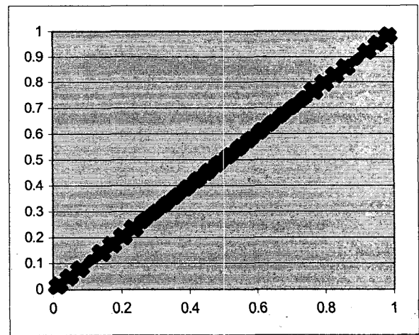
Figure 5: Same as Figure 4 Except Coordinates 47 & 48.
