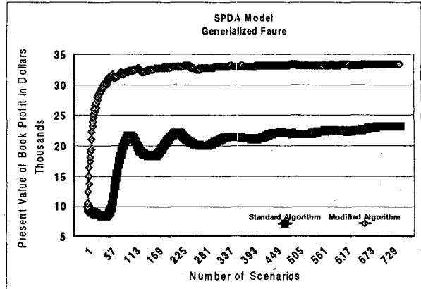
Figure 9: Generalized Faure with and without Leaping.
