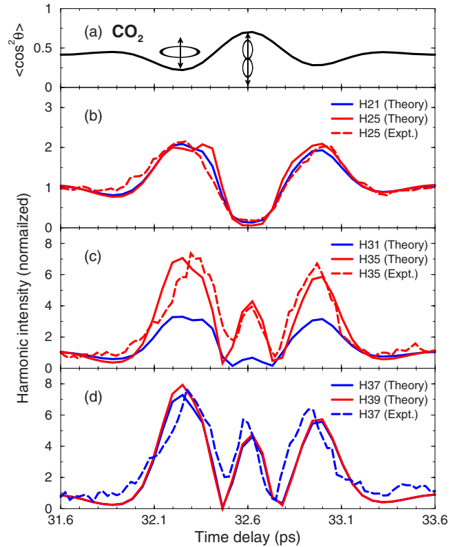
FIG. 11. (Color online) Normalized HHG yield (vs isotropically distributed molecules) from \text{CO}_2 for selected harmonics as function of pump-probe delay time near 3/4-revival. The experimental data are taken from Zhou et al. [16]. Theoretical results were obtained with laser parameters taken from [16]. The alignment parameter \langle \cos^2 \theta \rangle is also plotted for reference in the top panel.
