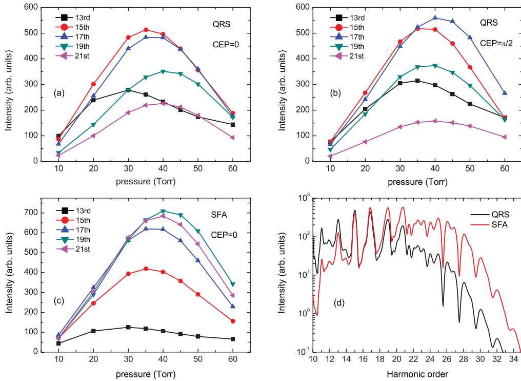
FIG. 3. (Color online) The harmonic intensity of Ar as a function of gas pressure for different orders from 13rd to 21st in the plateau for (a) \text{CEP} = 0 and (b) \text{CEP} = \pi/2 obtained by QRS. The laser peak intensity at focus is 2 \times 10^{14} \text{ W/cm}^2 , the other parameters are the same as those in simulation 1 in Fig. 1. (c) The same as (a) but obtained by SFA. (d) Comparison of HHG spectra obtained by QRS [black (dark gray) line] and SFA [red (light gray) line] for a pressure of 30 Torr and \text{CEP} = 0 .
